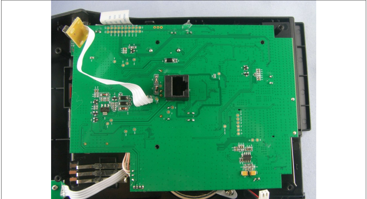
Exhibits Internal Photos_ZTU-9702MWD Board layout side view
