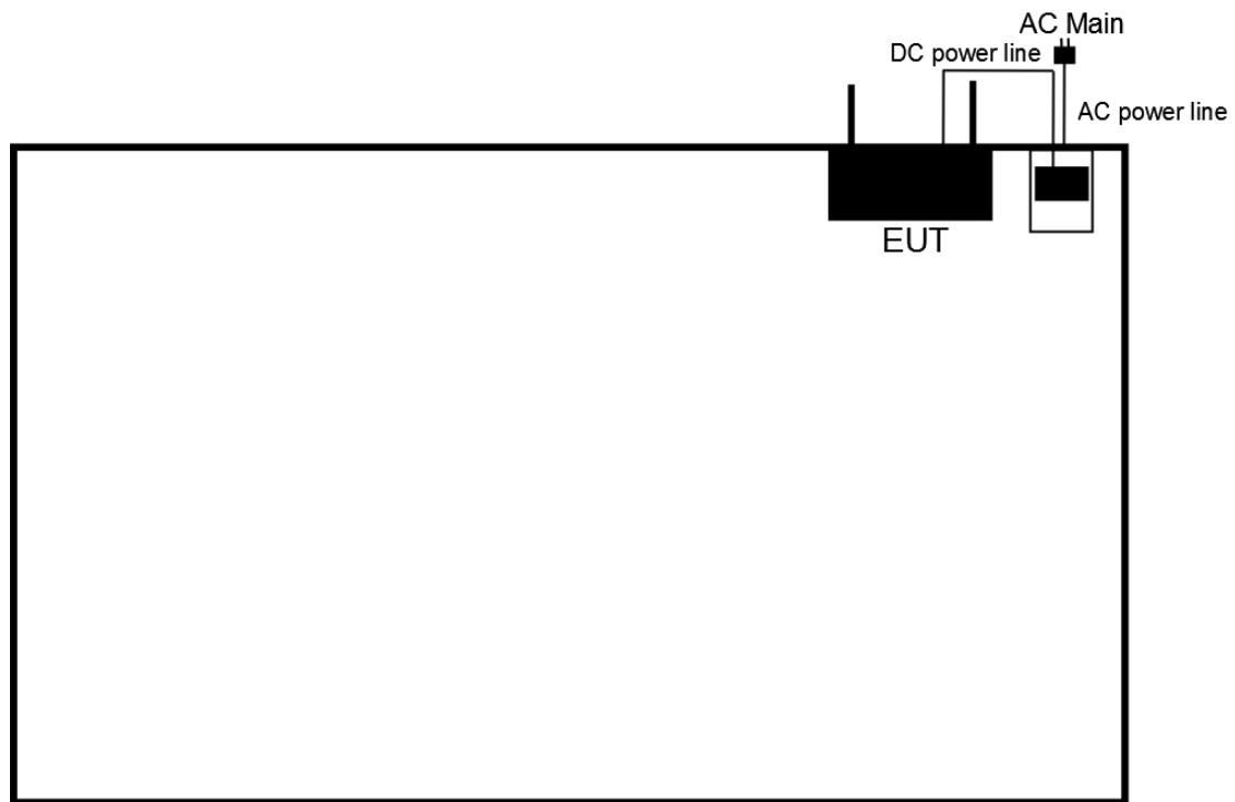
Test Setup Diagram - Radiated Emission Test
