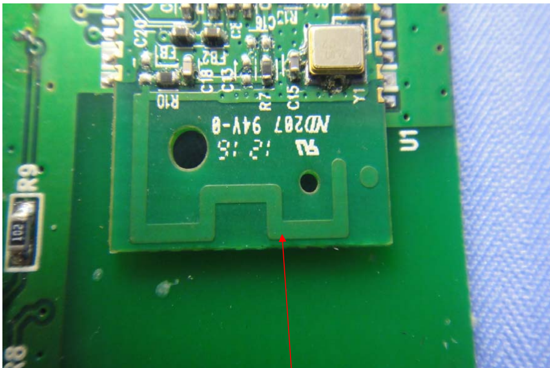
Printed Antenna
