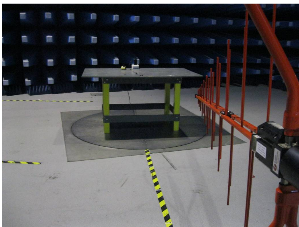
Radiated Emission Rear View (30MHz-1GHz)
