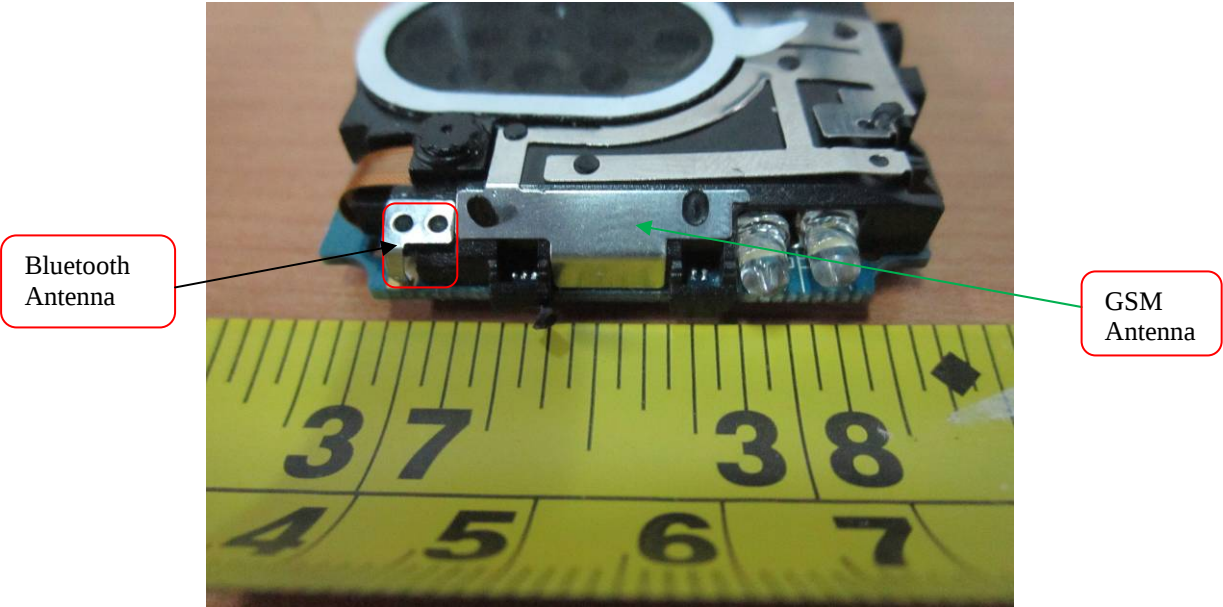
PCB Board view
