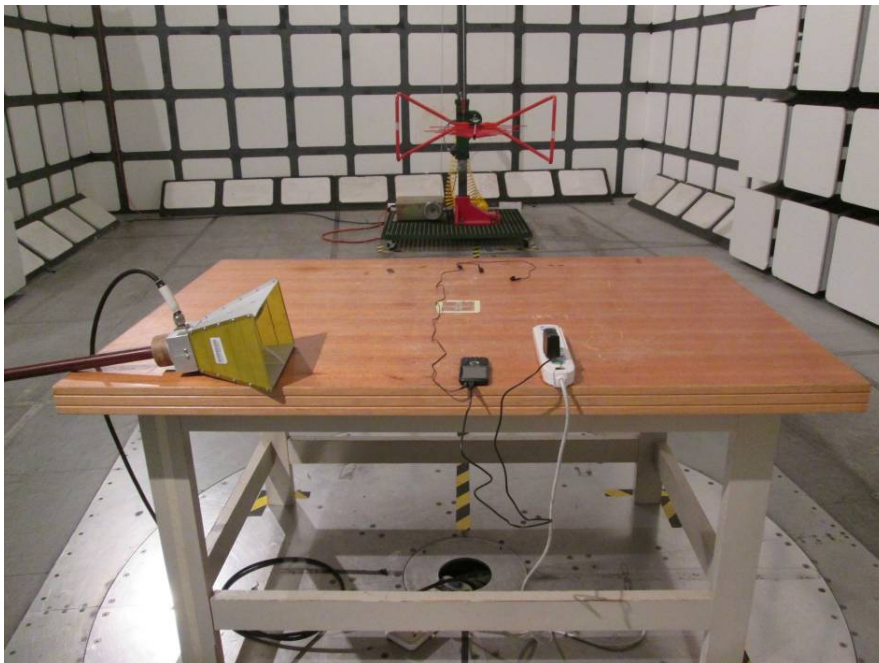
Radiated Emissions (30-1000 MHz) – Rear View
