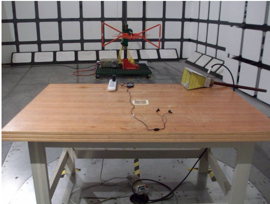
Radiated Emissions (30-1000 MHz) - Front View
