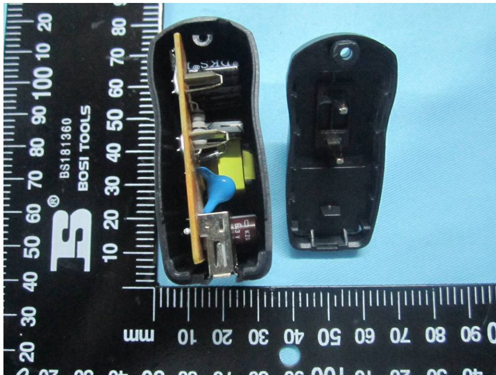
Adapter Cover Off – Front View
