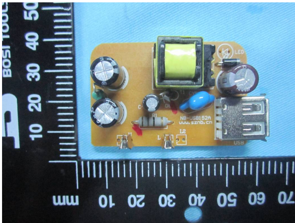
Adapter Mainboard - Front View
