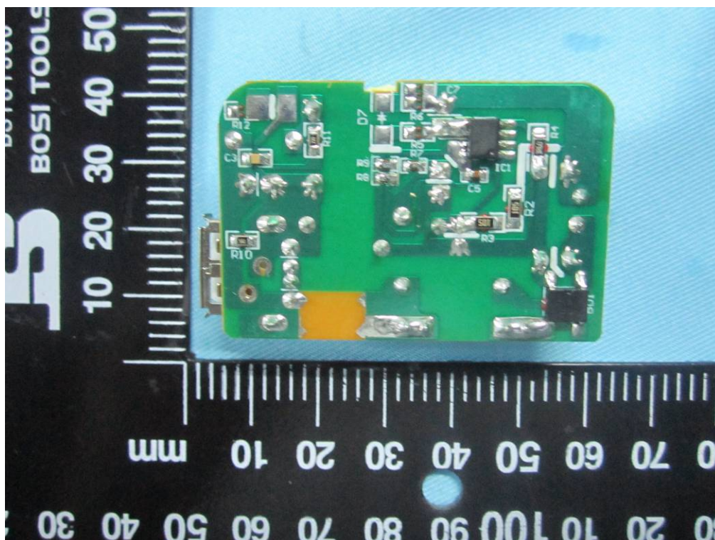
Adapter Mainboard - Rear View
