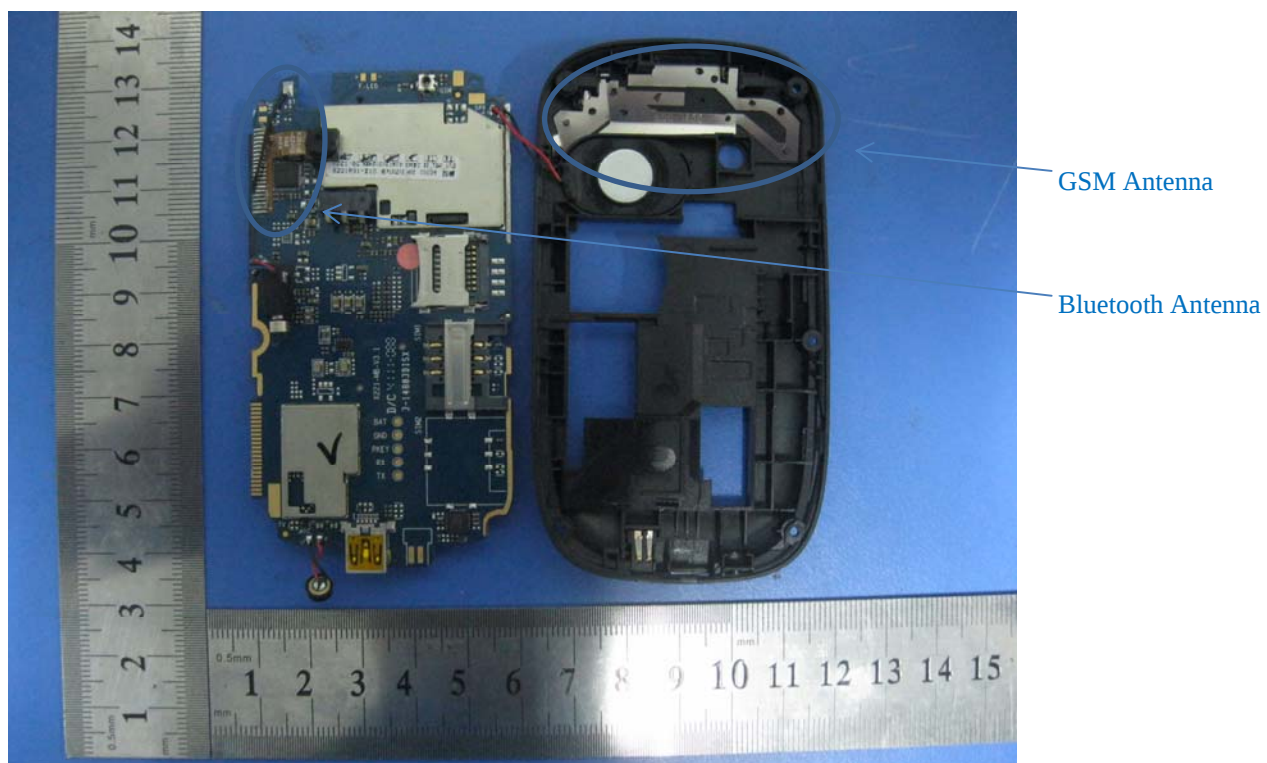
Antenna - Top View
