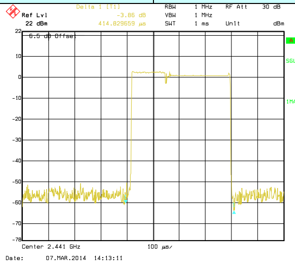
2-DH1
