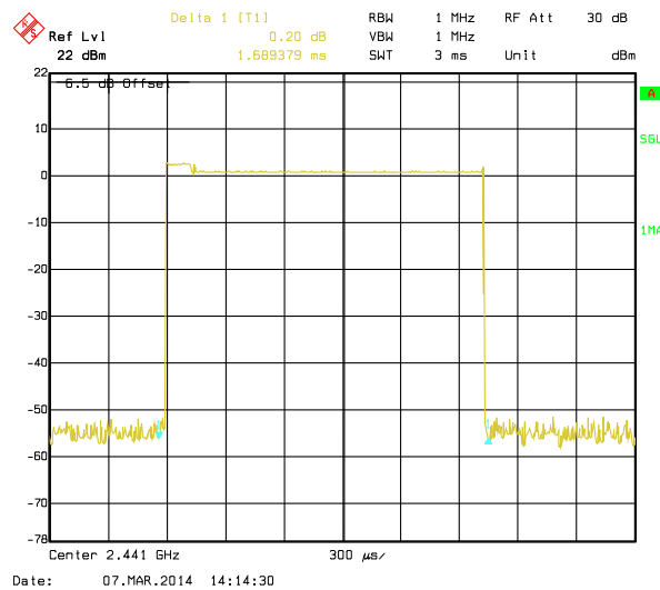
2-DH3
