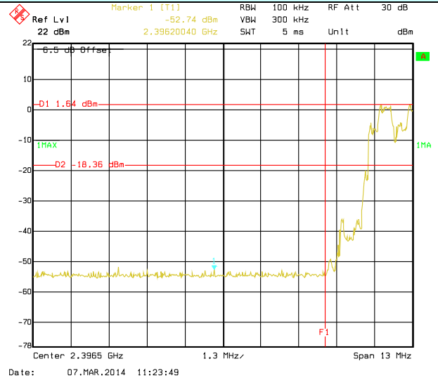
Hopping mode
