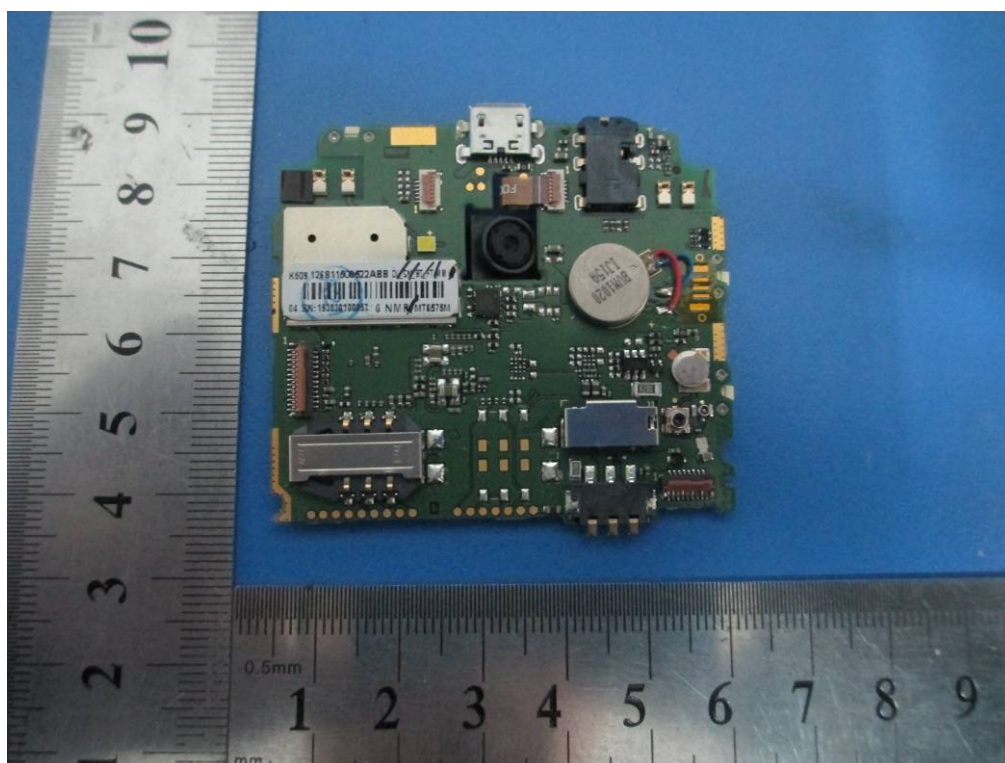
Top - PCB 1#
