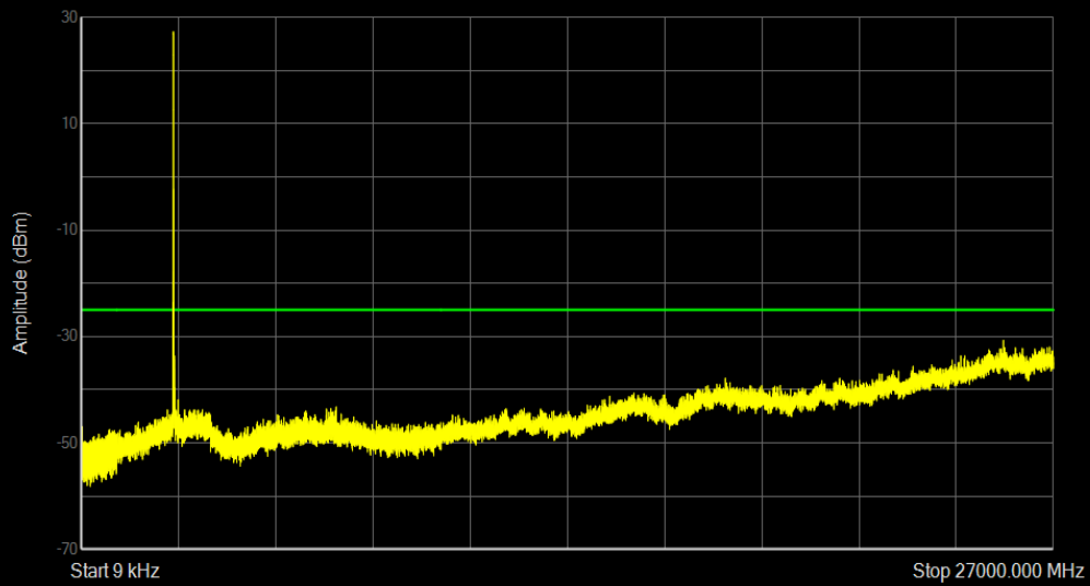
Band38 QPSK BW=15MHz Channel=37825 RB Size=1 Position=#0
