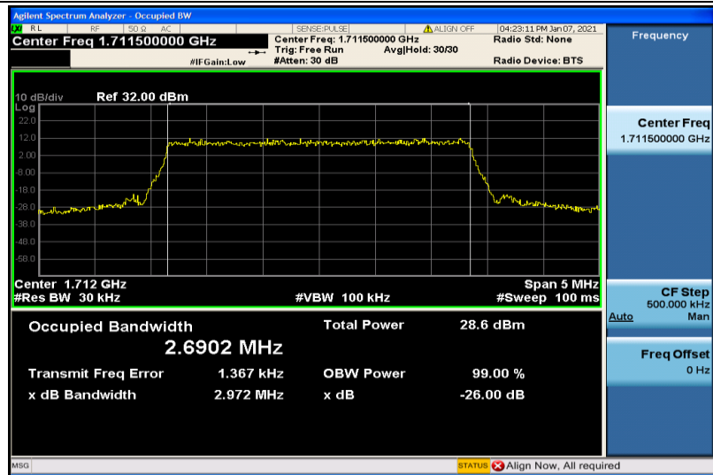
Band4-3MHz-QPSK-19965-15RB#0-2.6902
