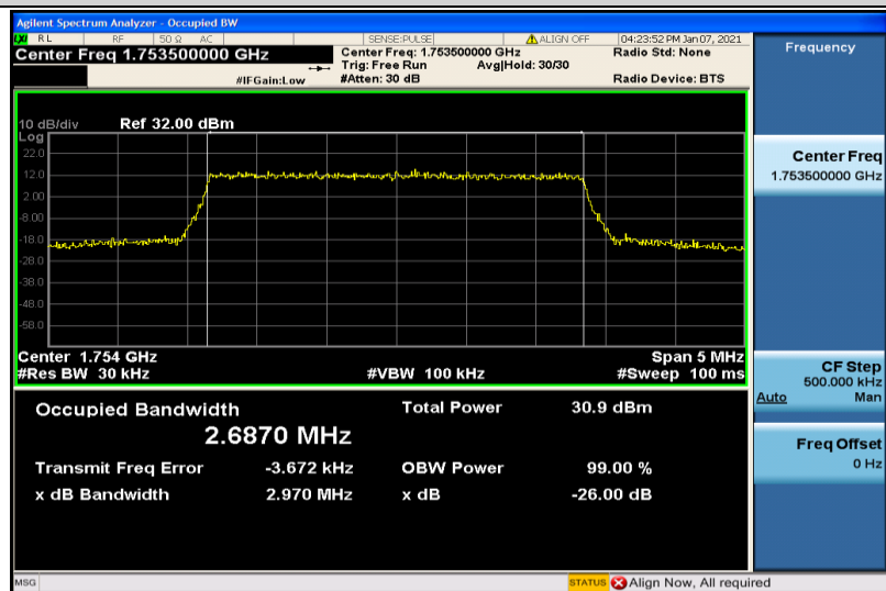
Band4-3MHz-QPSK-20385-15RB#0-2.6870
