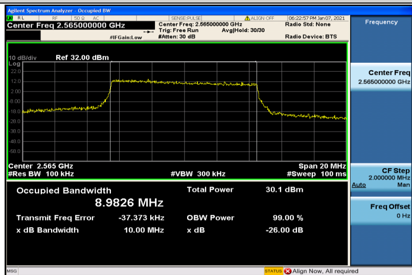
Band7-10MHz-16QAM-21400-50RB#0-8.9826
