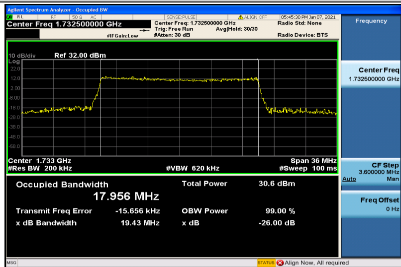
Band4-20MHz-16QAM-20175-100RB#0-17.956
