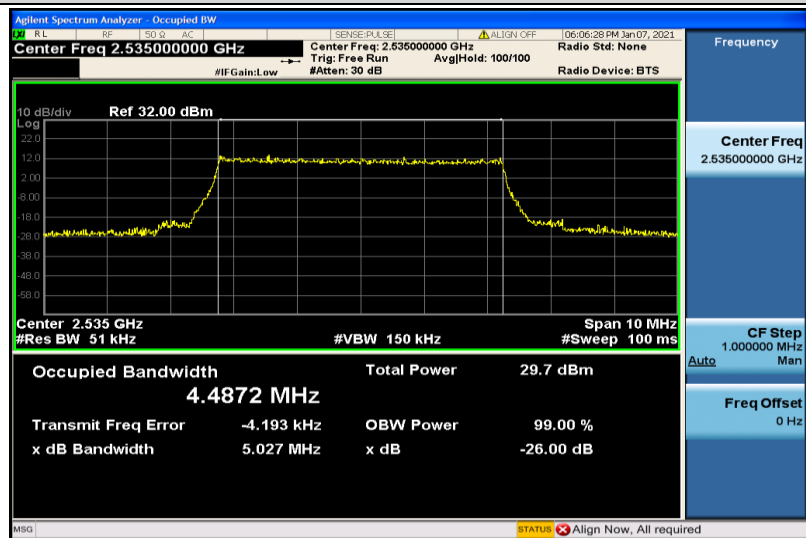
Band7-5MHz-QPSK-21100-25RB#0-4.4872
