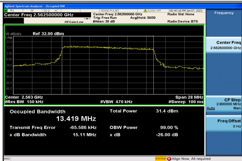
Band7-15MHz-QPSK-21375-75RB#0-13.419
