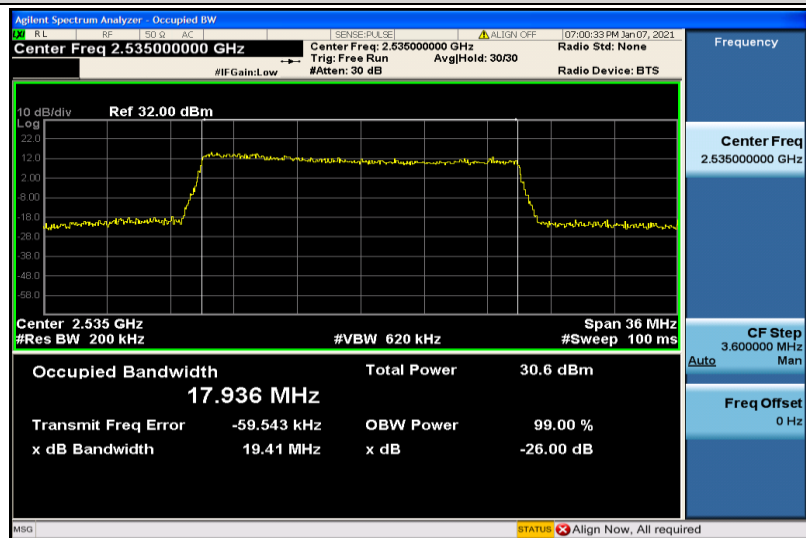
Band7-20MHz-QPSK-21100-100RB#0-17.936
