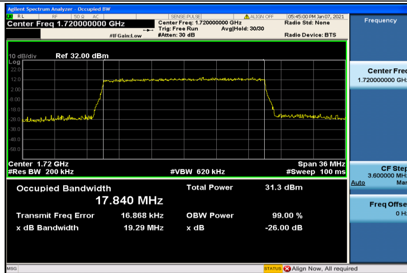
Band4-20MHz-QPSK-20050-100RB#0-17.840
