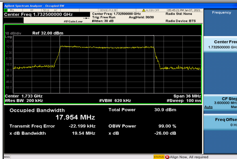
Band4-20MHz-QPSK-20175-100RB#0-17.954
