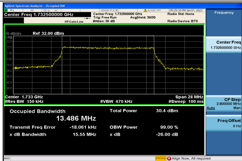
Band4-15MHz-16QAM-20175-75RB#0-13.486
