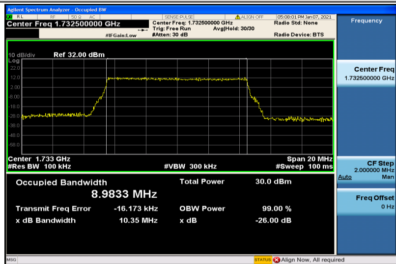
Band4-10MHz-QPSK-20175-50RB#0-8.9833
