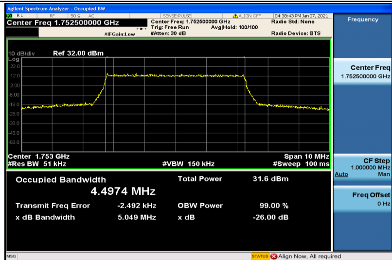
Band4-5MHz-QPSK-20375-25RB#0-4.4974
