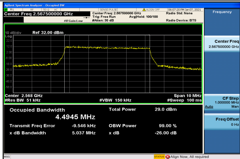
Band7-5MHz-16QAM-21425-25RB#0-4.4945
