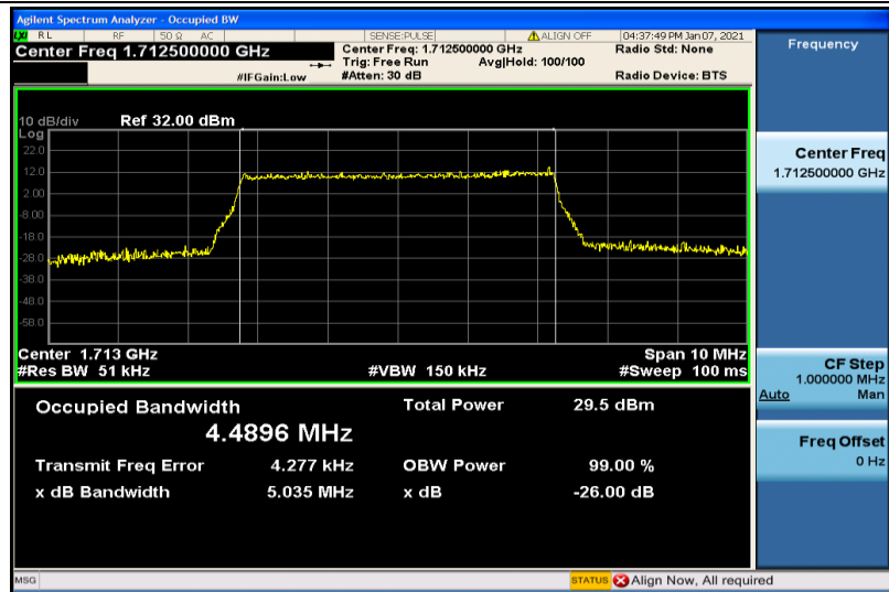
Band4-5MHz-16QAM-19975-25RB#0-4.4896
