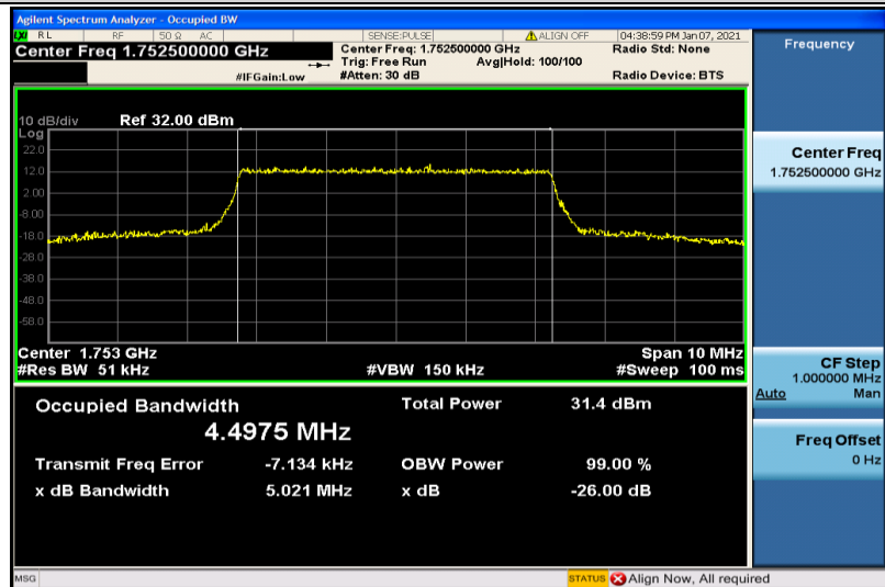
Band4-5MHz-16QAM-20375-25RB#0-4.4975
