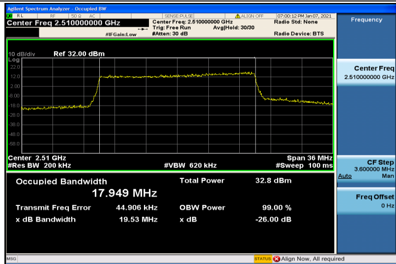
Band7-20MHz-QPSK-20850-100RB#0-17.949
