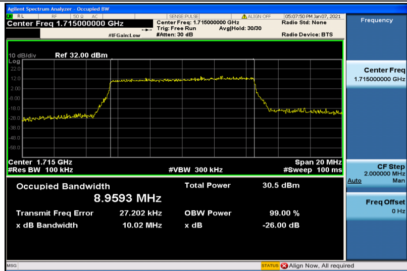
Band4-10MHz-16QAM-20000-50RB#0-8.9593
