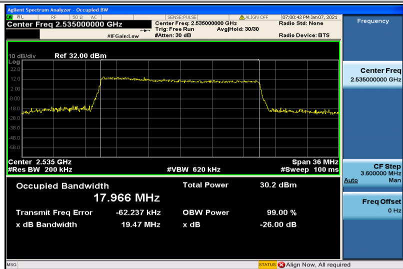
Band7-20MHz-16QAM-21100-100RB#0-17.966
