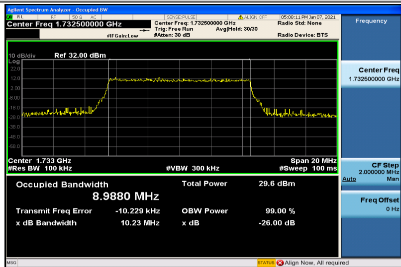
Band4-10MHz-16QAM-20175-50RB#0-8.9880
