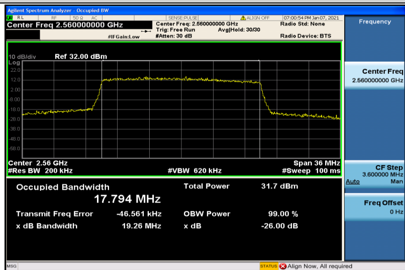
Band7-20MHz-QPSK-21350-100RB#0-17.794
