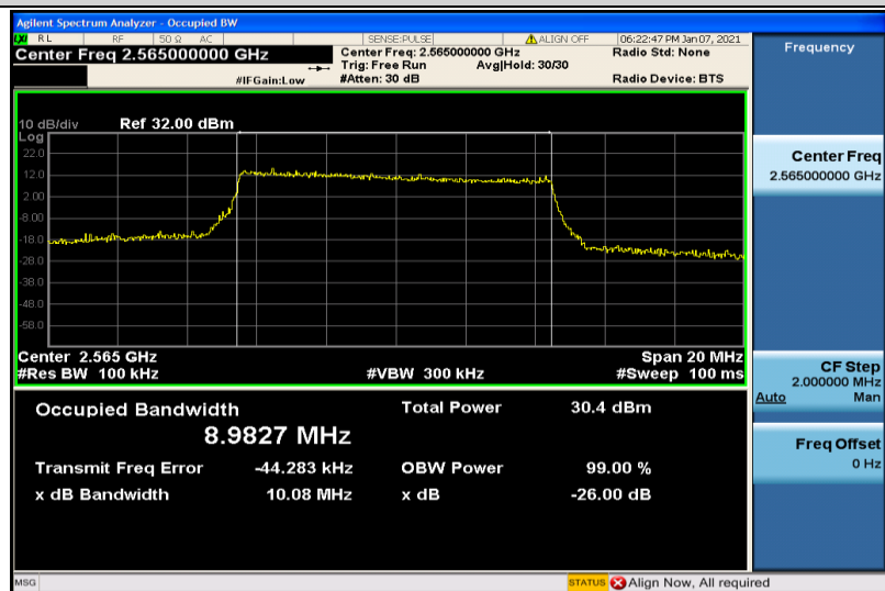
Band7-10MHz-QPSK-21400-50RB#0-8.9827
