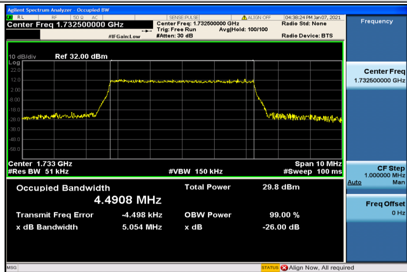
Band4-5MHz-16QAM-20175-25RB#0-4.4908
