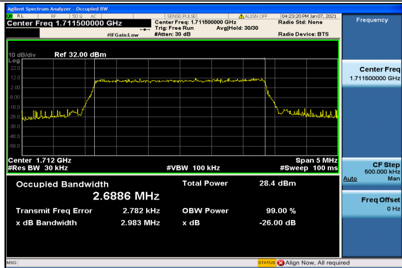
Band4-3MHz-16QAM-19965-15RB#0-2.6886
