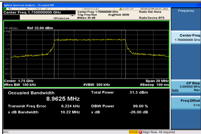
Band4-10MHz-16QAM-20350-50RB#0-8.9625
