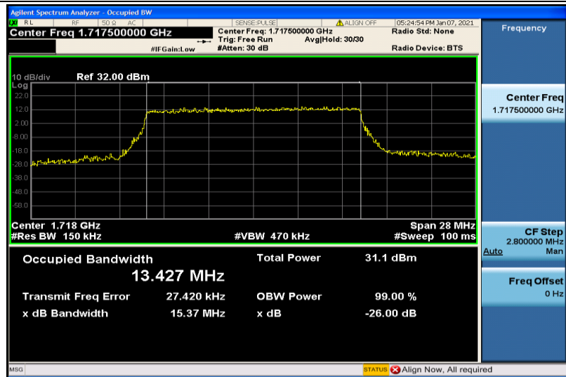
Band4-15MHz-16QAM-20025-75RB#0-13.427
