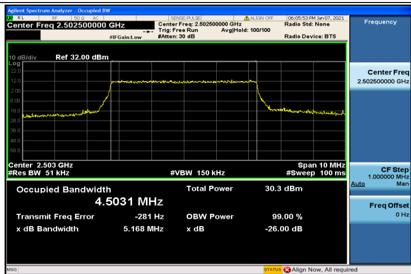
Band7-5MHz-QPSK-20775-25RB#0-4.5031
