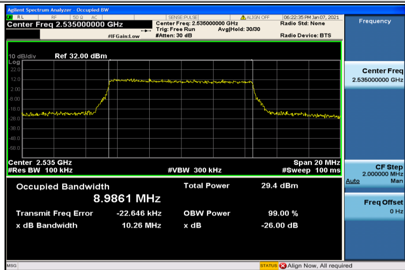
Band7-10MHz-16QAM-21100-50RB#0-8.9861
