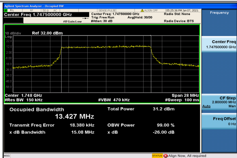
Band4-15MHz-16QAM-20325-75RB#0-13.427
