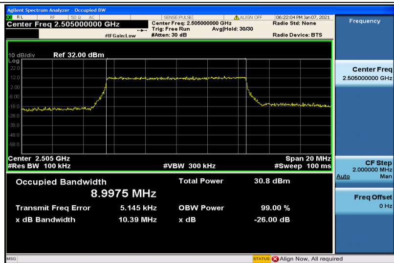
Band7-10MHz-QPSK-20800-50RB#0-8.9975
