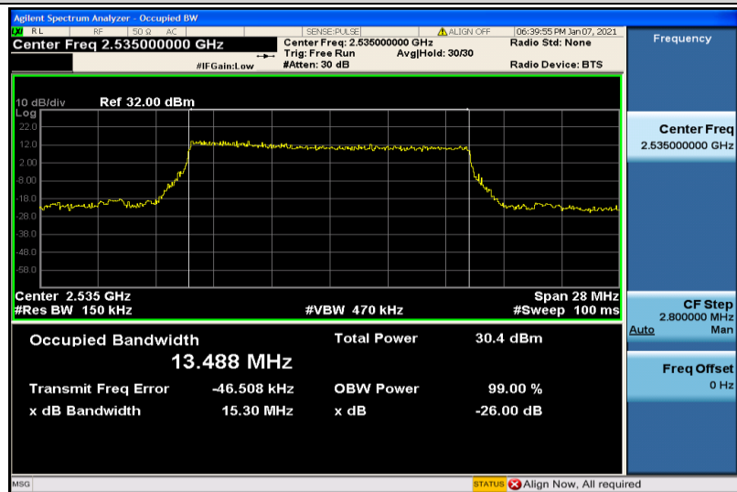
Band7-15MHz-QPSK-21100-75RB#0-13.488
