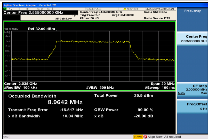
Band7-10MHz-QPSK-21100-50RB#0-8.9642
