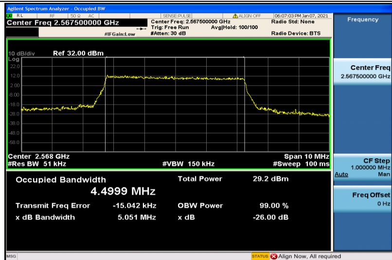
Band7-5MHz-QPSK-21425-25RB#0-4.4999
