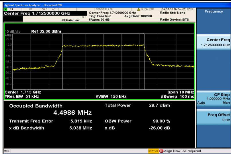
Band4-5MHz-QPSK-19975-25RB#0-4.4986
