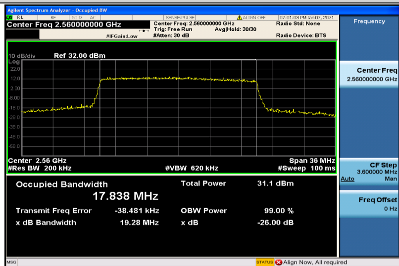
Band7-20MHz-16QAM-21350-100RB#0-17.838
