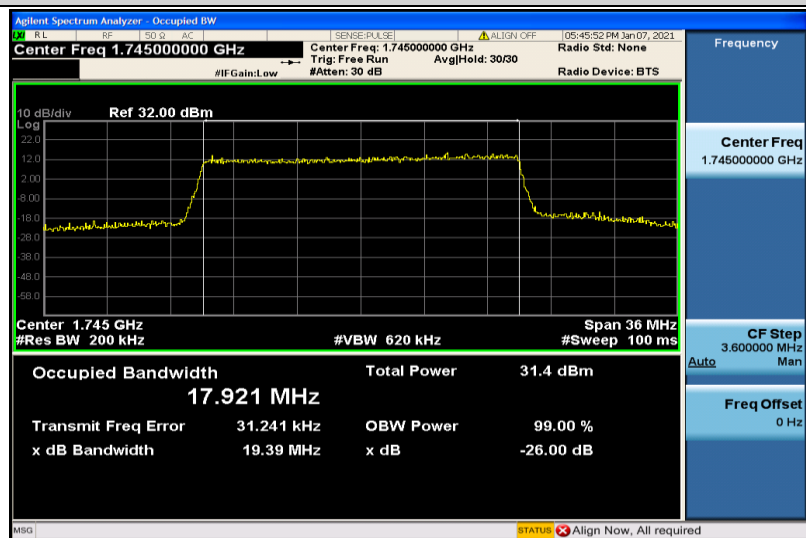
Band4-20MHz-16QAM-20300-100RB#0-17.921
