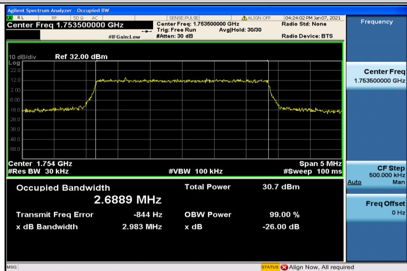
Band4-3MHz-16QAM-20385-15RB#0-2.6889
