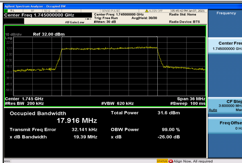
Band4-20MHz-QPSK-20300-100RB#0-17.916
