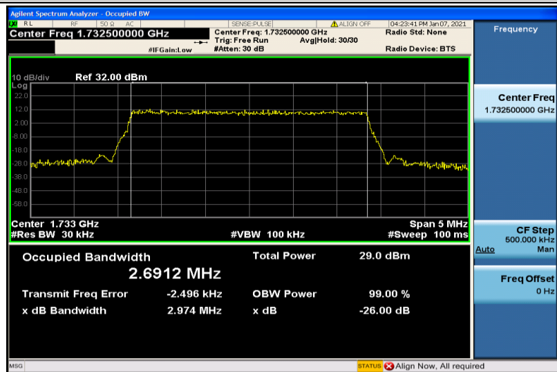
Band4-3MHz-16QAM-20175-15RB#0-2.6912
