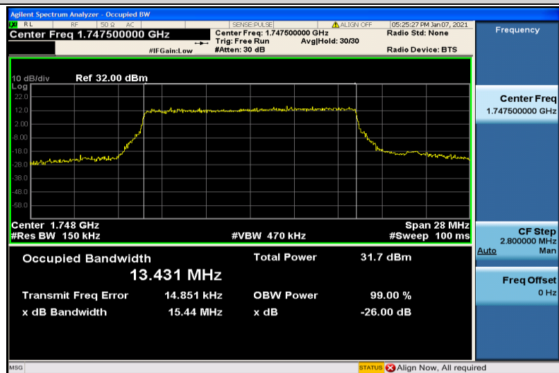
Band4-15MHz-QPSK-20325-75RB#0-13.431
