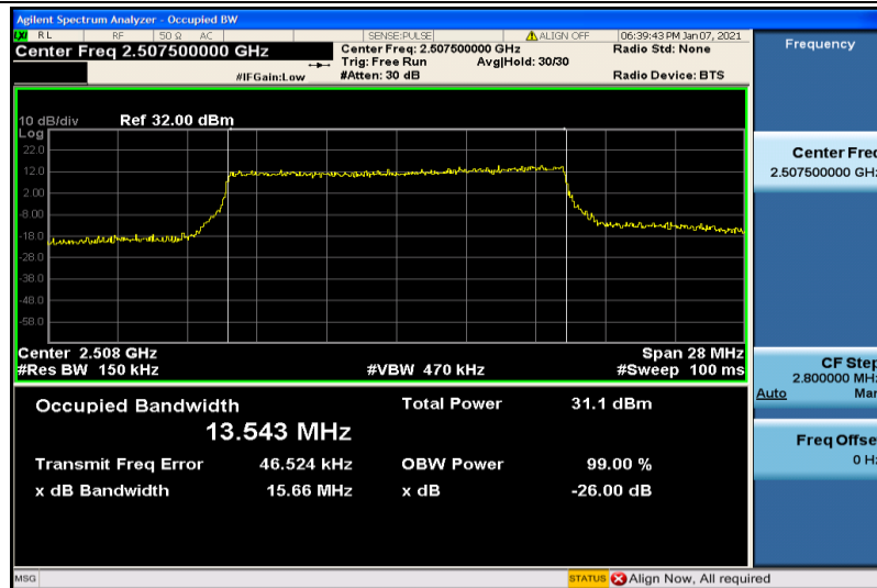
Band7-15MHz-16QAM-20825-75RB#0-13.543
