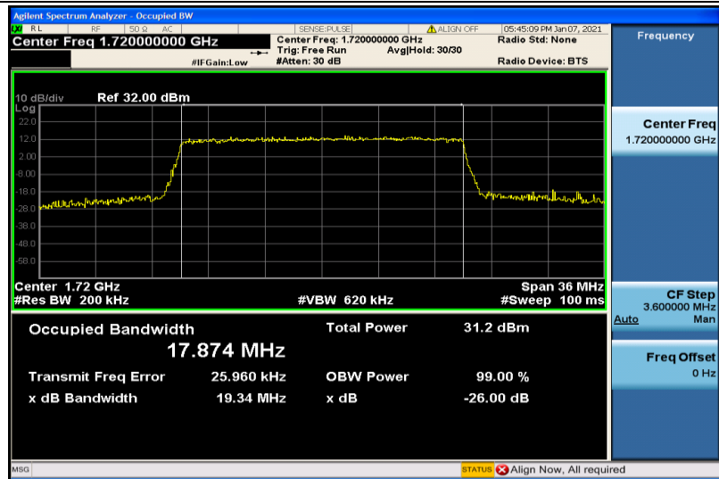
Band4-20MHz-16QAM-20050-100RB#0-17.874
