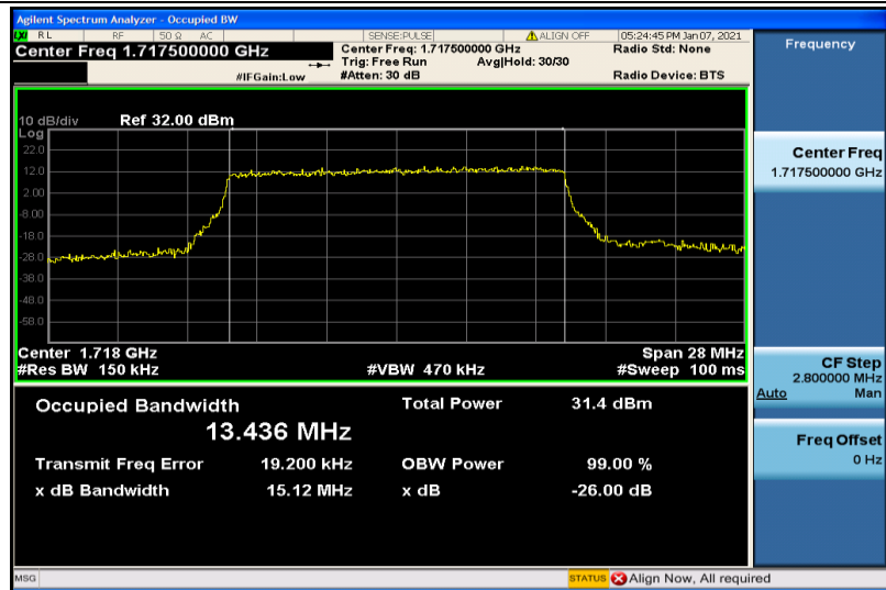
Band4-15MHz-QPSK-20025-75RB#0-13.436
