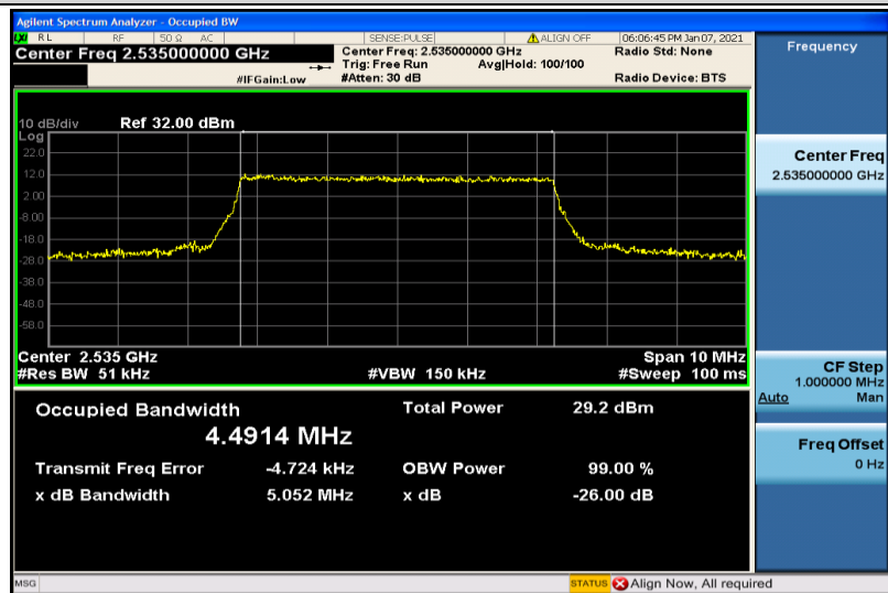
Band7-5MHz-16QAM-21100-25RB#0-4.4914
