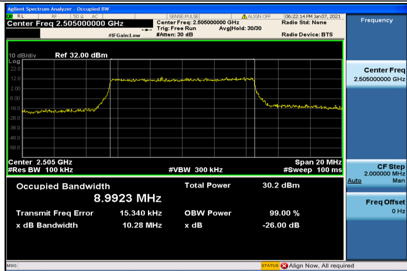
Band7-10MHz-16QAM-20800-50RB#0-8.9923
