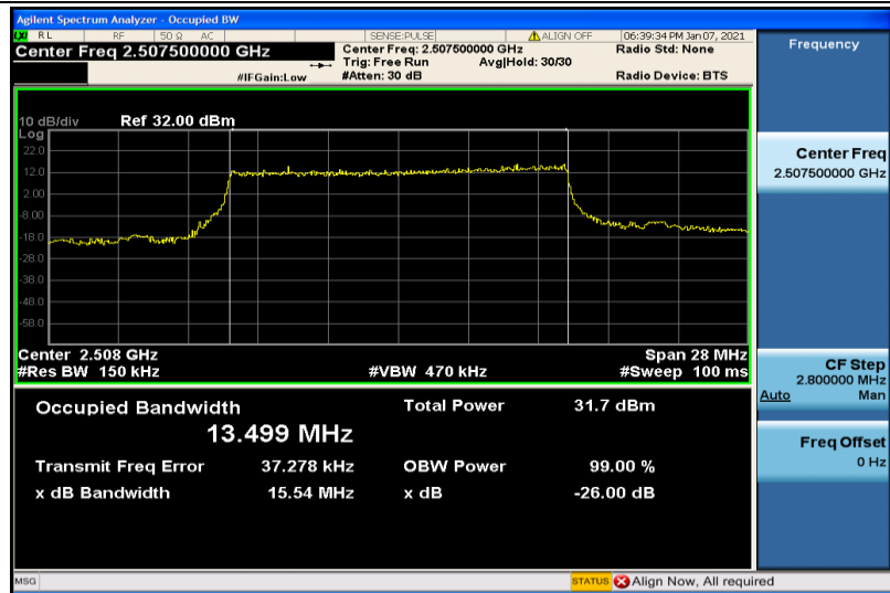
Band7-15MHz-QPSK-20825-75RB#0-13.499
