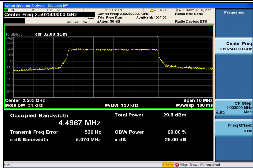
Band7-5MHz-16QAM-20775-25RB#0-4.4967
