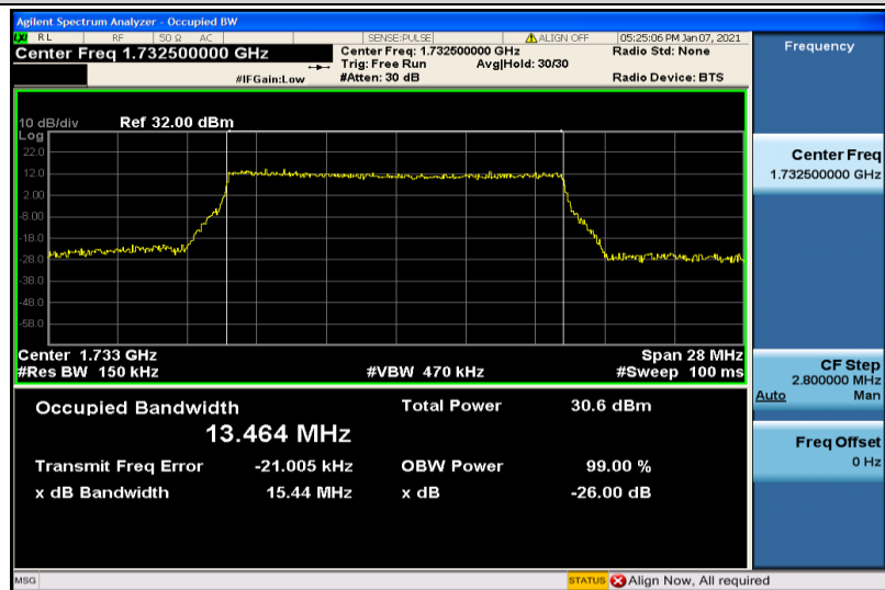
Band4-15MHz-QPSK-20175-75RB#0-13.464
