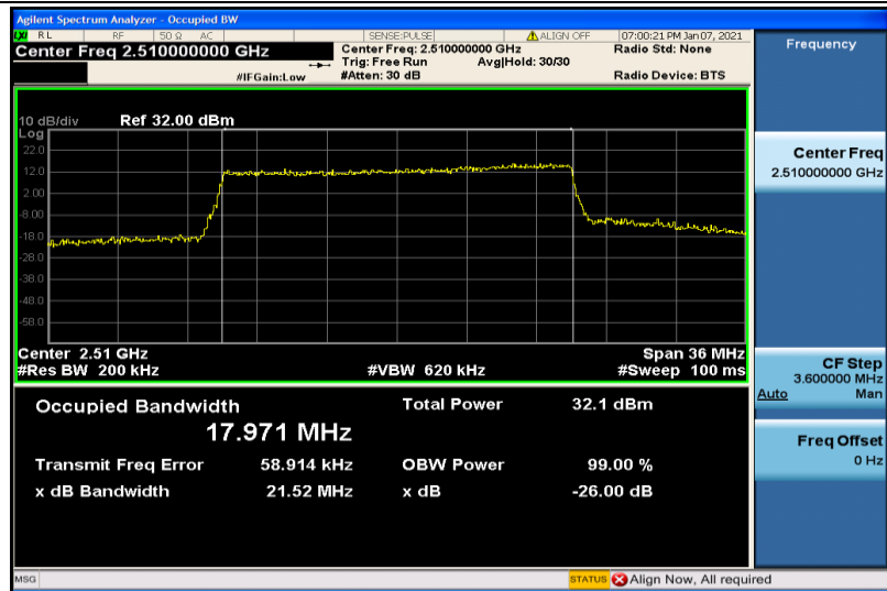
Band7-20MHz-16QAM-20850-100RB#0-17.971
