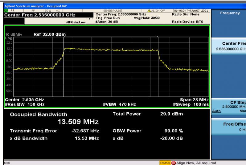
Band7-15MHz-16QAM-21100-75RB#0-13.509
