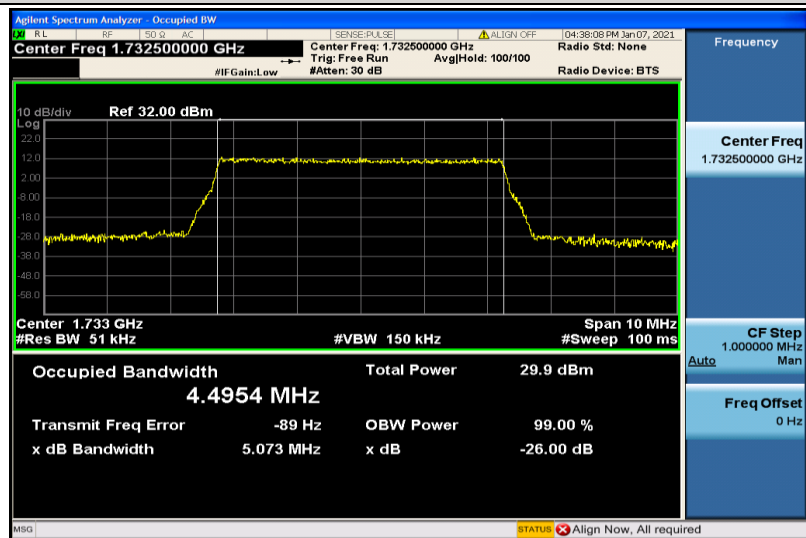
Band4-5MHz-QPSK-20175-25RB#0-4.4954
