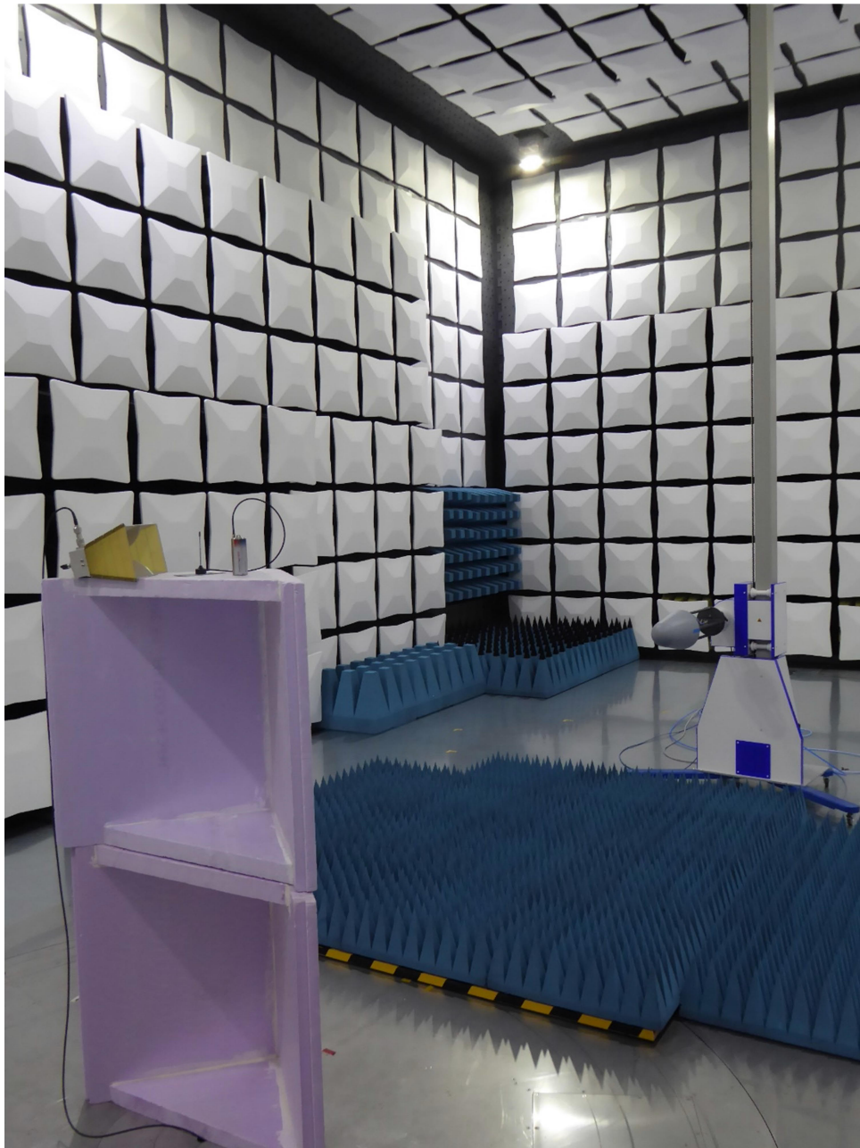
Test Setup SAC from 1 GHz to 18 GHz
