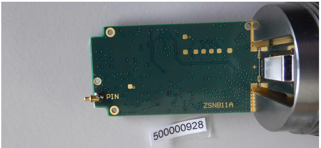
PCB of IoT Leak Logger (host device), bottom view, label removed
