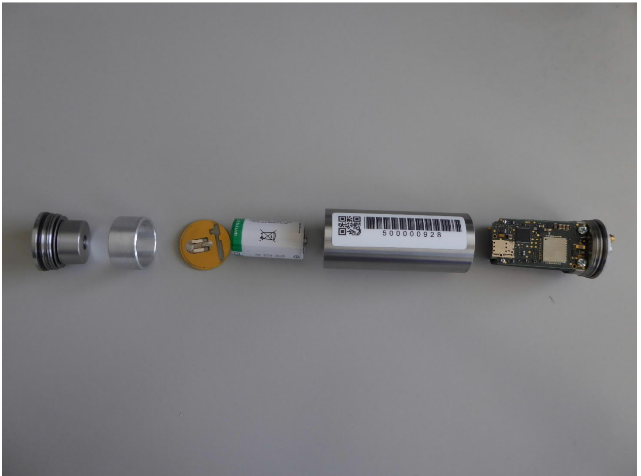
IoT Leak Logger, assembly view
