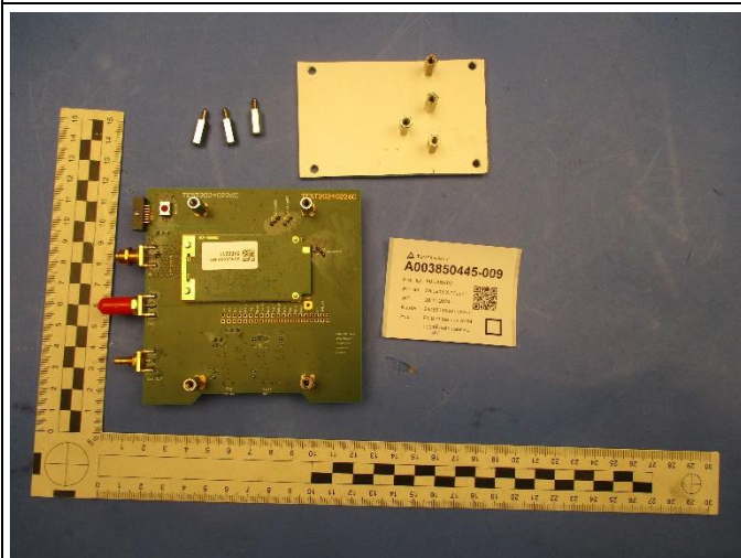
Evaluation Board
