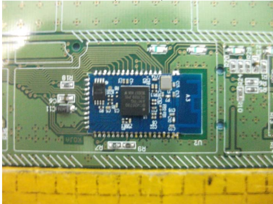
Figure 7 PCB of the EUT-Front View(BT Module)
