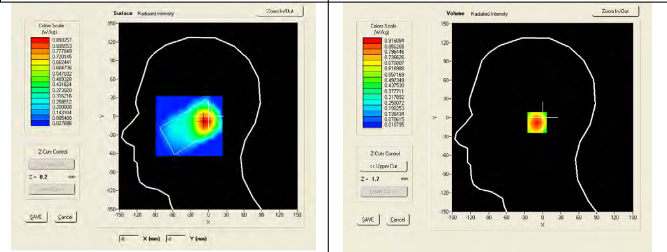
SAR, Z Axis Scan (X = -5, Y = -8)
