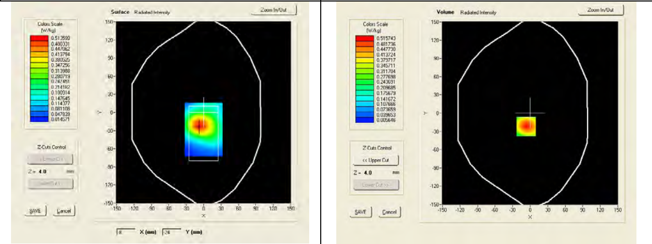
SAR, Z Axis Scan (X = -7, Y = -22)
