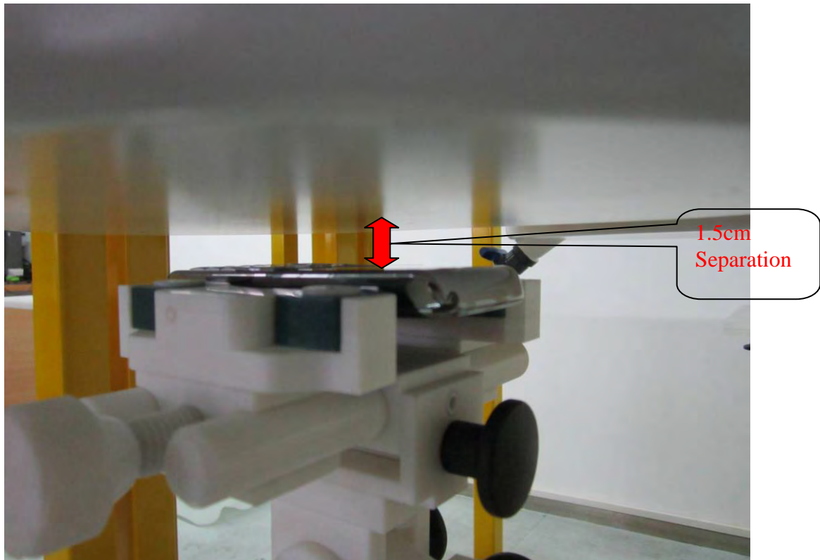
Body Setup Photo (LCD UP)
