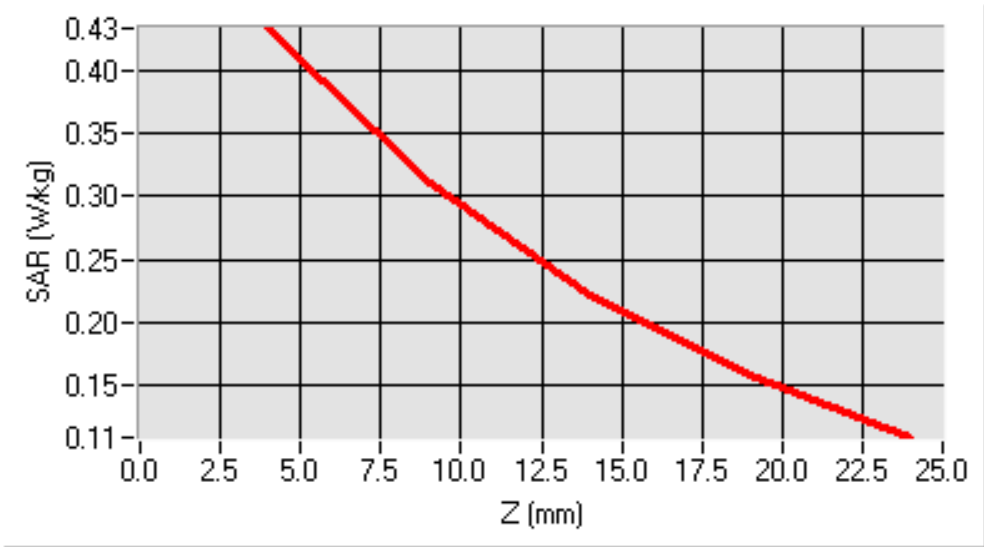
SAR, Z Axis Scan (X = -14, Y = 1)
