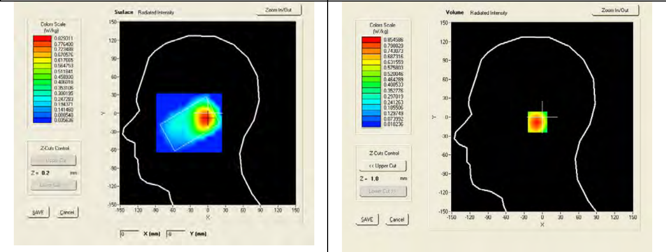
SAR, Z Axis Scan (X = -3, Y = -8)
