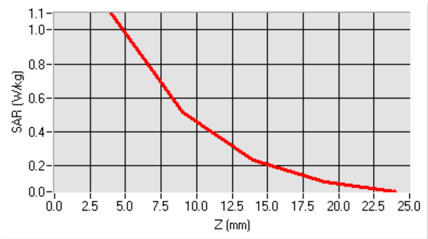
SAR, Z Axis Scan (X = -3, Y = -8)
