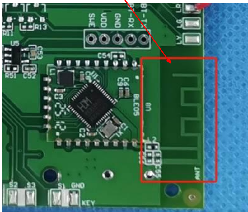
View of wireless antenna
