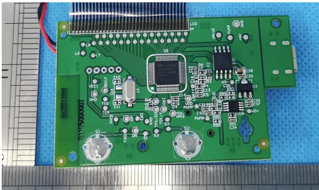
Inner circuit bottom view
