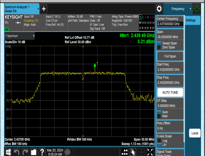
11N20SISO-Ant1-2437-0~Reference-PASS
