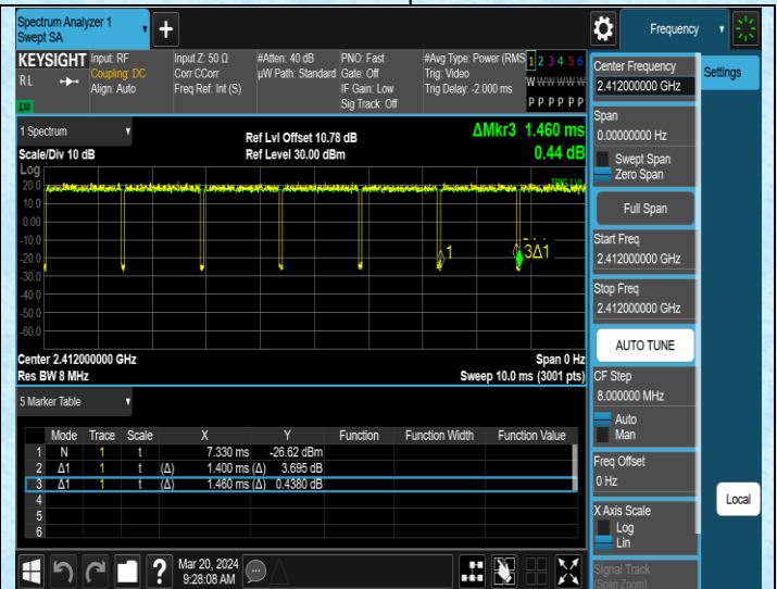
NTNV-11G-Ant1-2412
