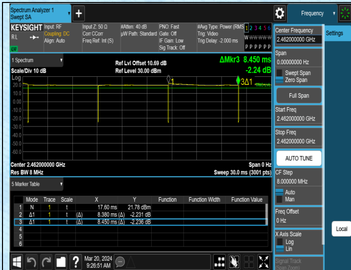
NTNV-11B-Ant1-2462
