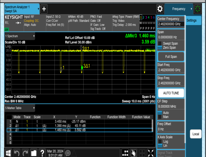
NTNV-11G-Ant1-2462
