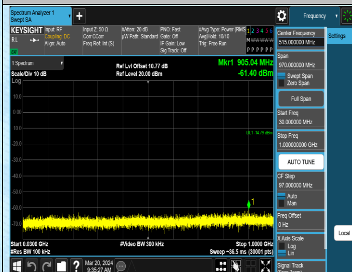
11N20SISO-Ant1-2437-30~1000-PASS
