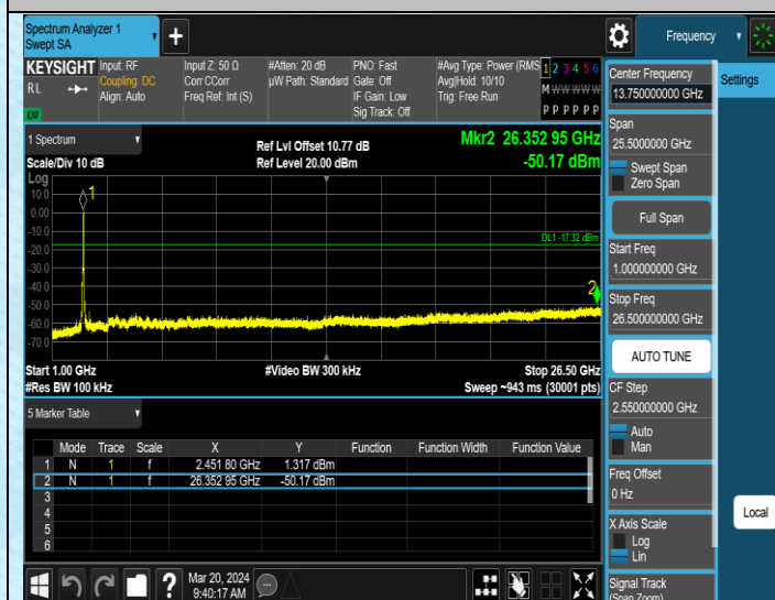
11N40SISO-Ant1-2437-1000~26500-PASS
