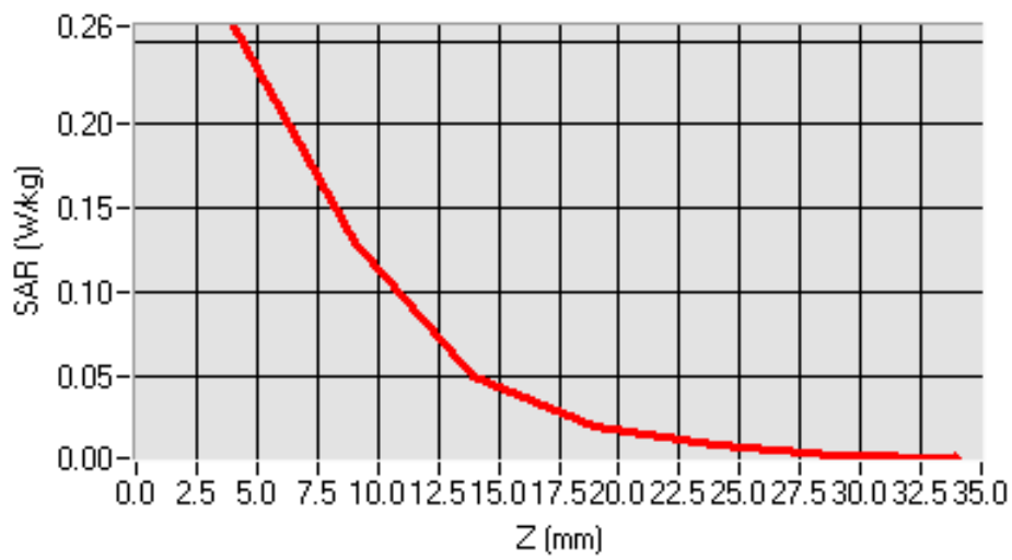
SAR, Z Axis Scan (X = -14, Y = 55)
