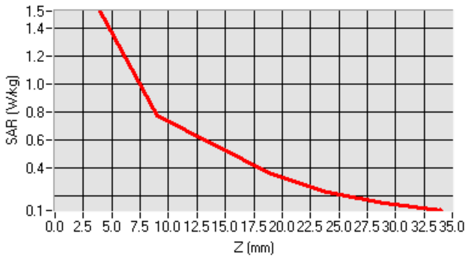
SAR, Z Axis Scan (X = 0, Y = 41)
