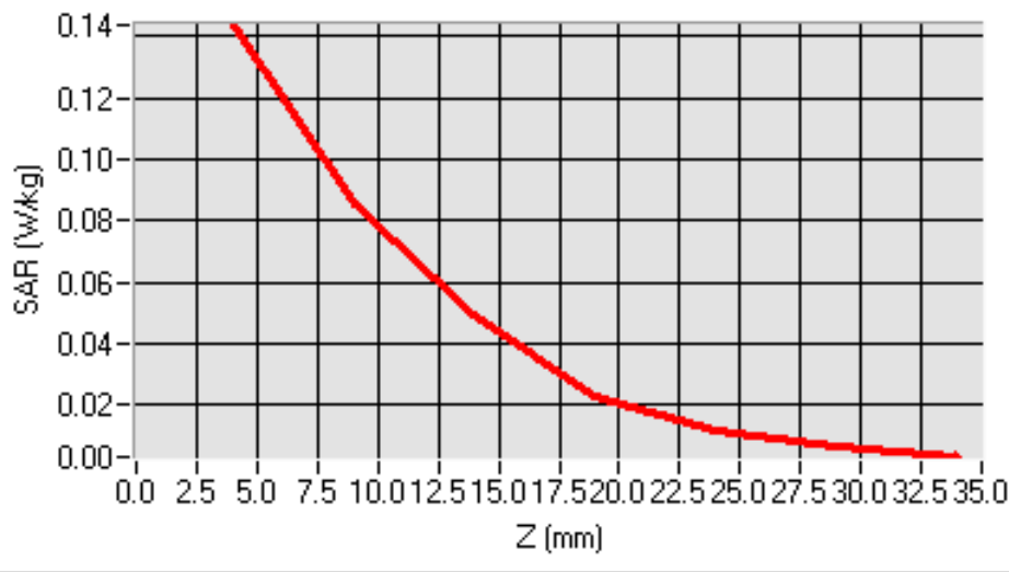
SAR, Z Axis Scan (X = -10, Y = 16)
