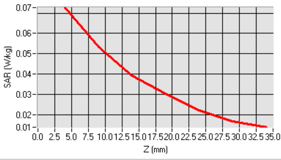
SAR, Z Axis Scan (X = -1, Y = -1)
