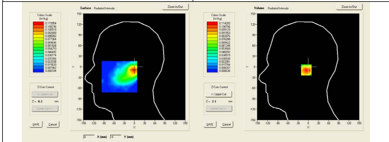
SAR, Z Axis Scan (X = -1, Y = -9)
