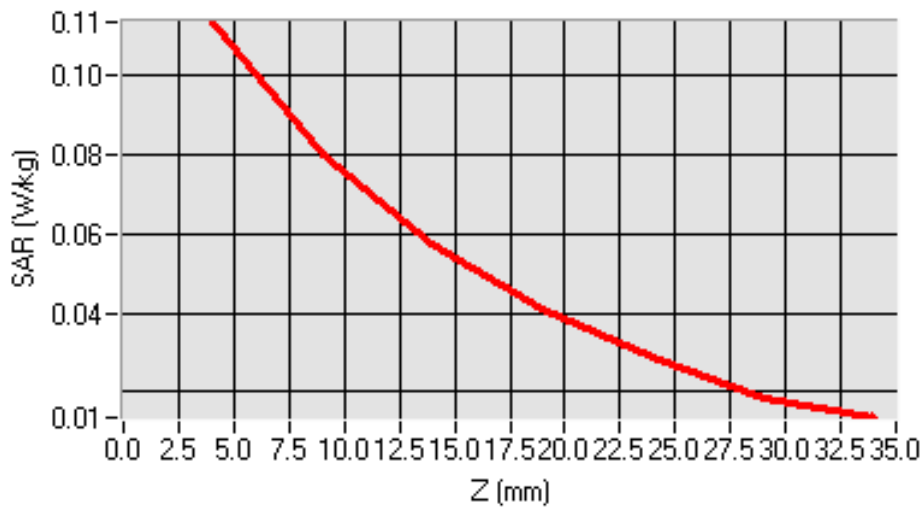
SAR, Z Axis Scan (X = 40, Y = 23)
