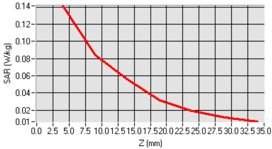
SAR, Z Axis Scan (X = 2, Y = -9)
