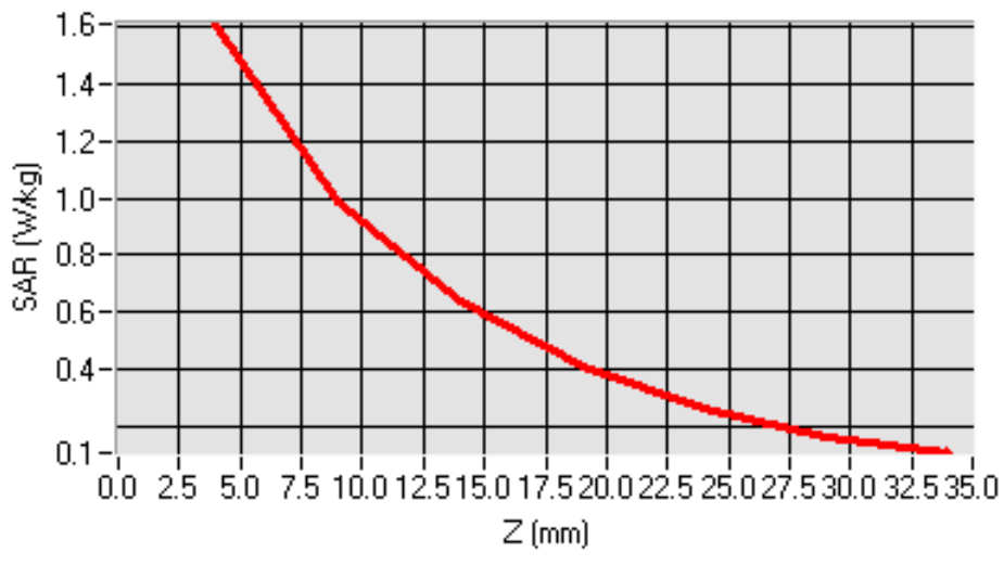
SAR, Z Axis Scan (X = 0, Y = 41)
