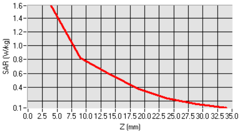
SAR, Z Axis Scan (X = 0, Y = 46)
