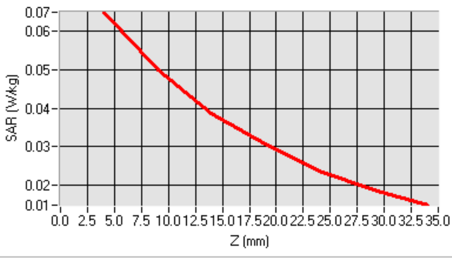
SAR, Z Axis Scan (X = -15, Y = -5)
