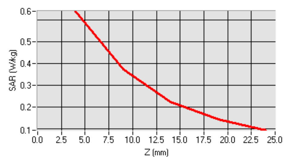
SAR, Z Axis Scan (X = 6, Y = -33)
