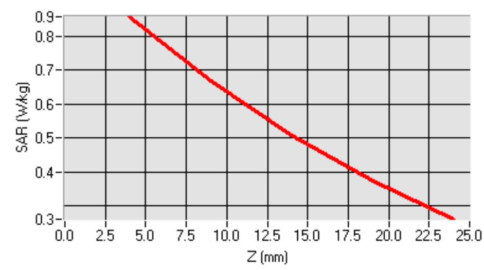
SAR, Z Axis Scan (X = -24, Y = -7)
