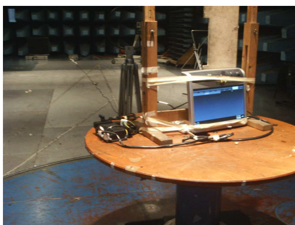
Loop antenna (9 kHz ÷ 30 MHz) measurement distance: 3 m
