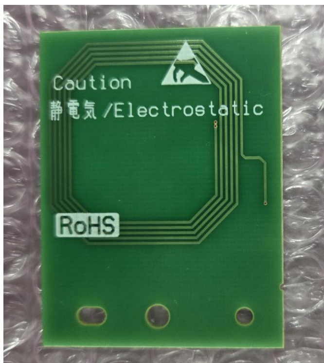
Antenna Board(Side B)
