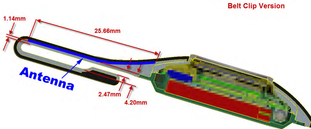
Figure 12-2 Internal cross-section drawing of MPERS LC130 showing antenna location
