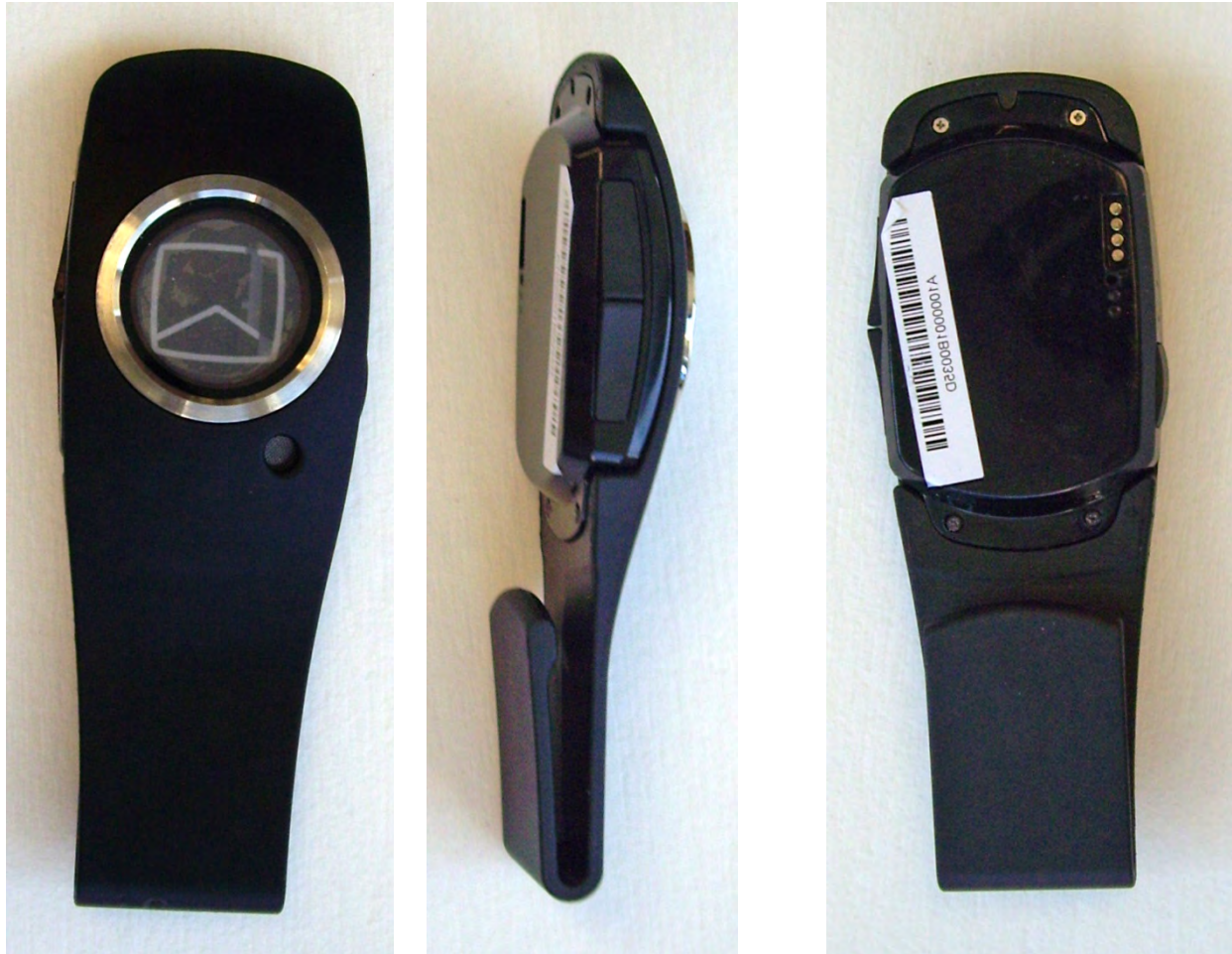
Figure 12-1 Front, Edge and Rear Views of MPERS LC130
