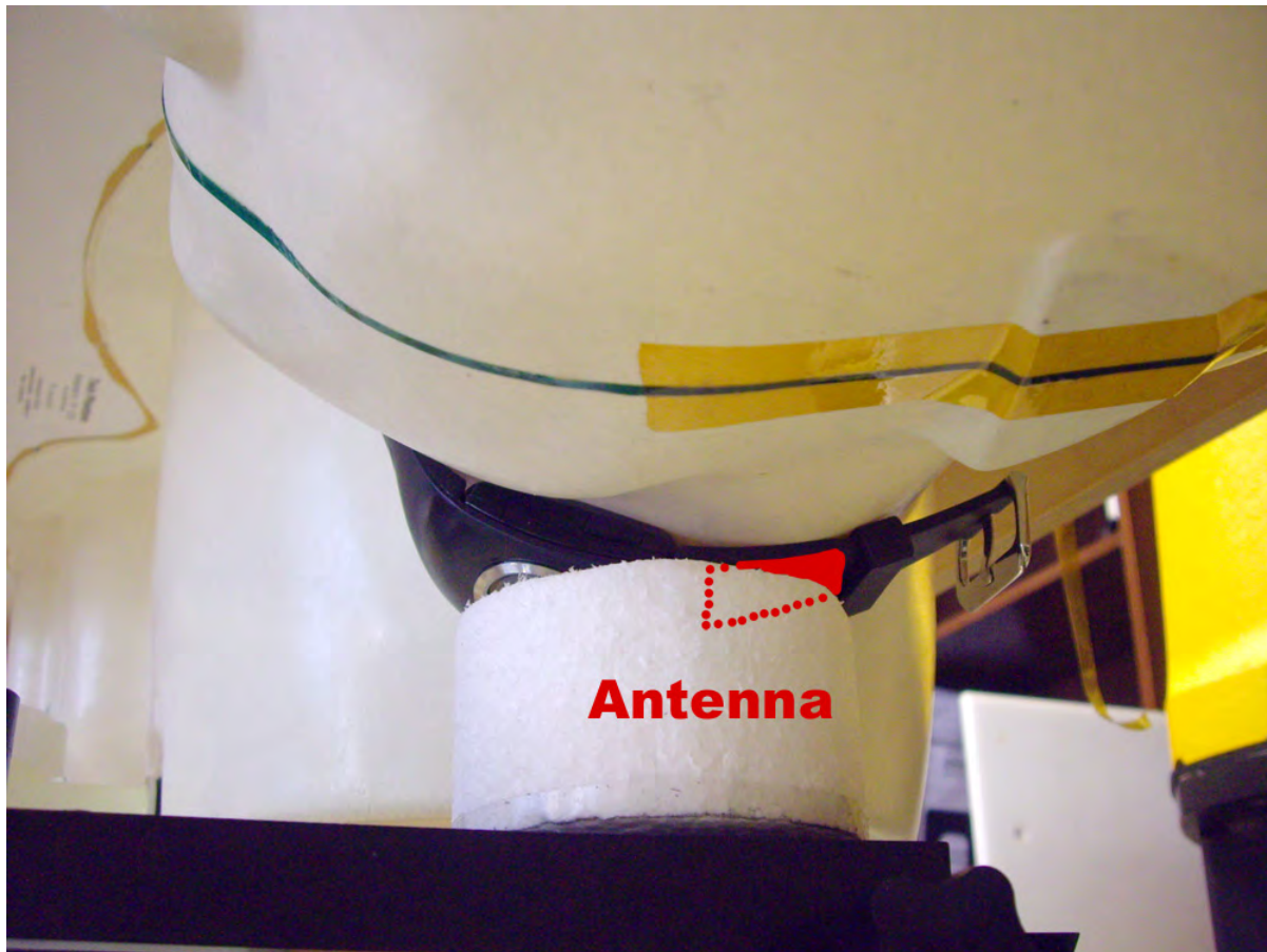
Figure 12-6 DUT rear toward phantom, 0 cm separation
