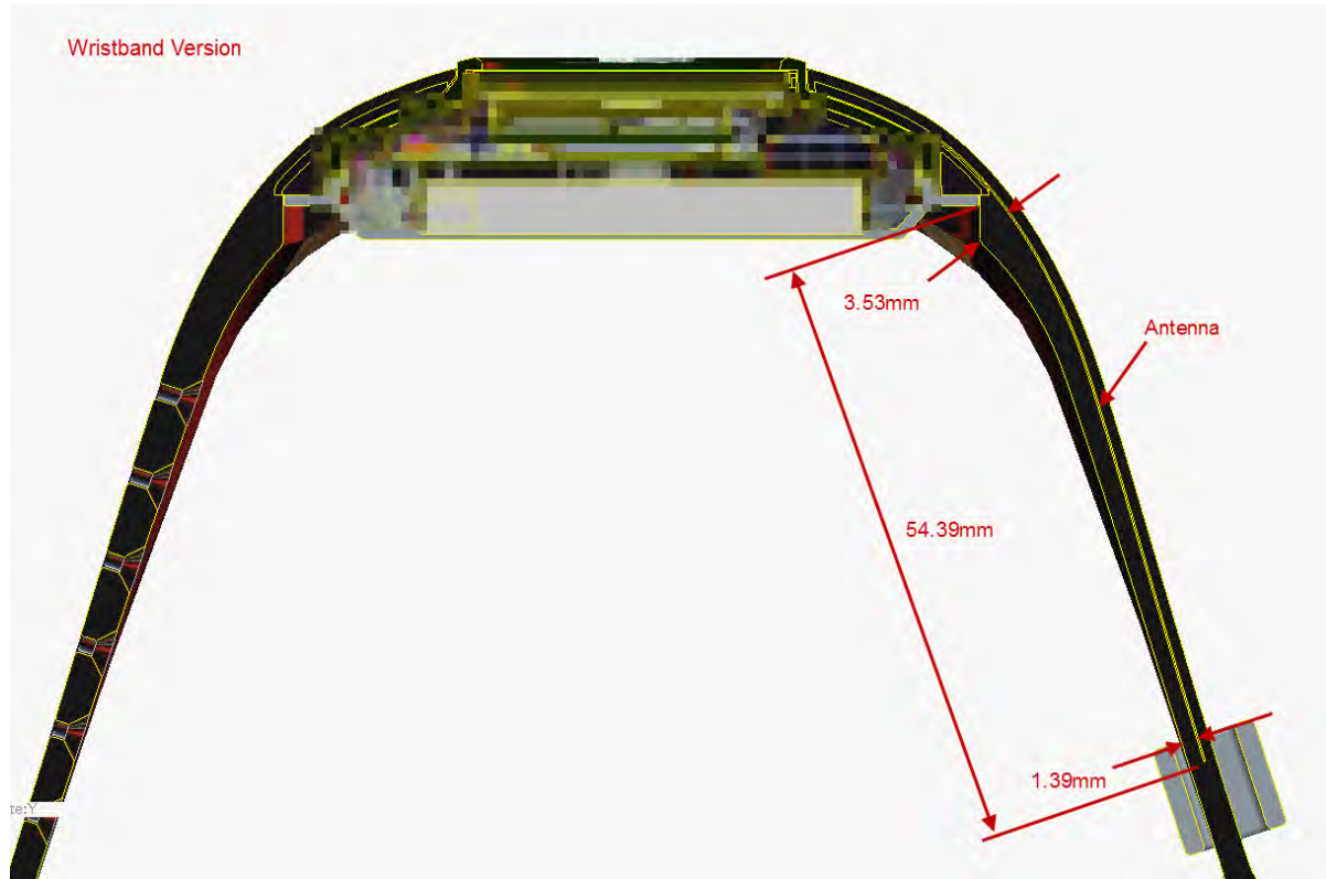
Figure 12-3 Internal cross-section drawing of MPERS LC120 showing antenna location
