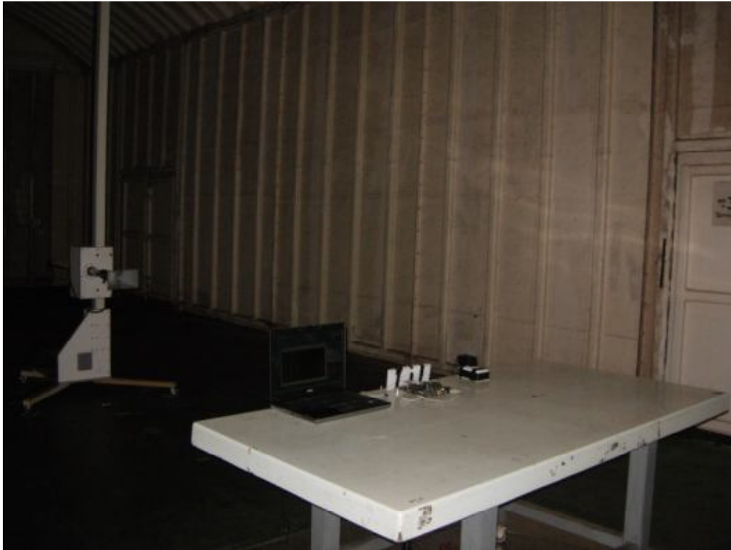
Back View of Radiated Test (Horn) - CX870-D60
