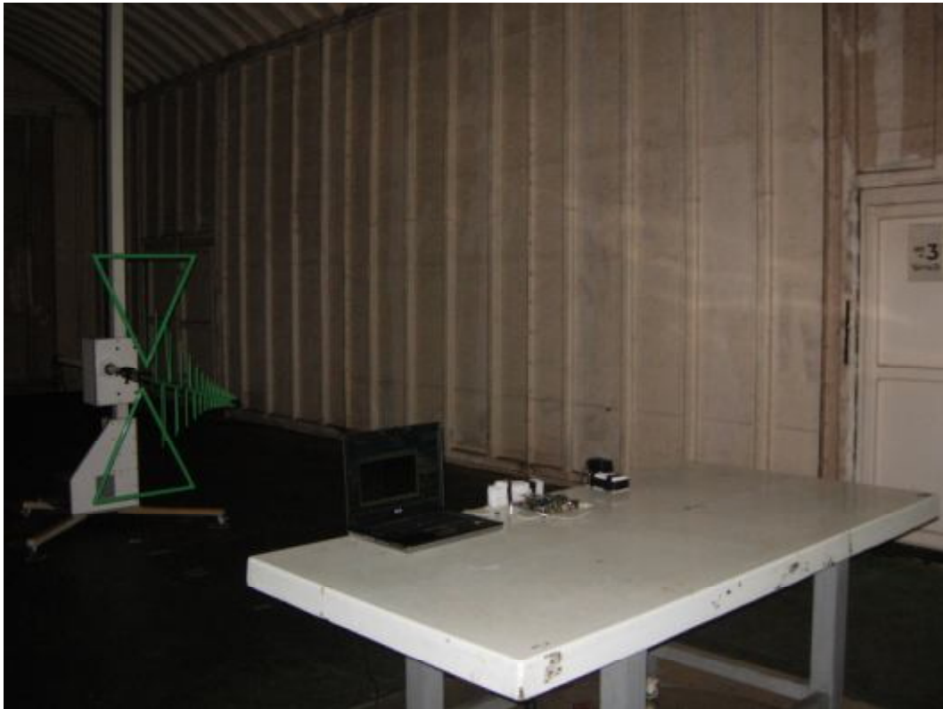
Back View of Radiated Test - CX870-D
