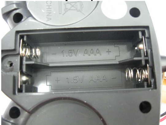
Battery compartment
