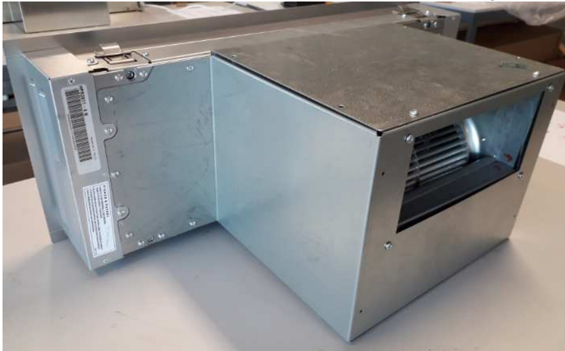
Transmitter located in side flange of rangehood (left of photo)
