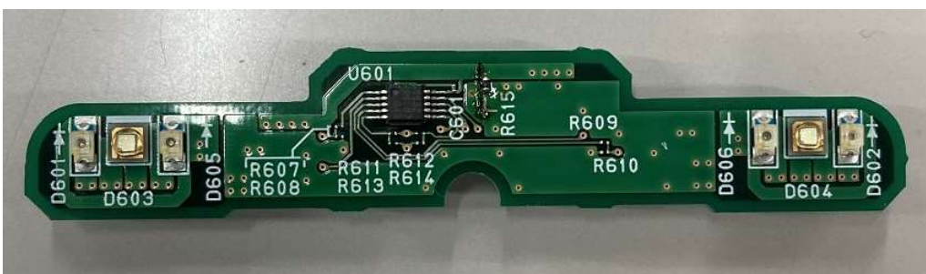
LED board_R front
