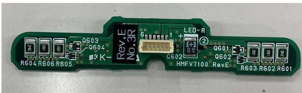
LED board_R back
