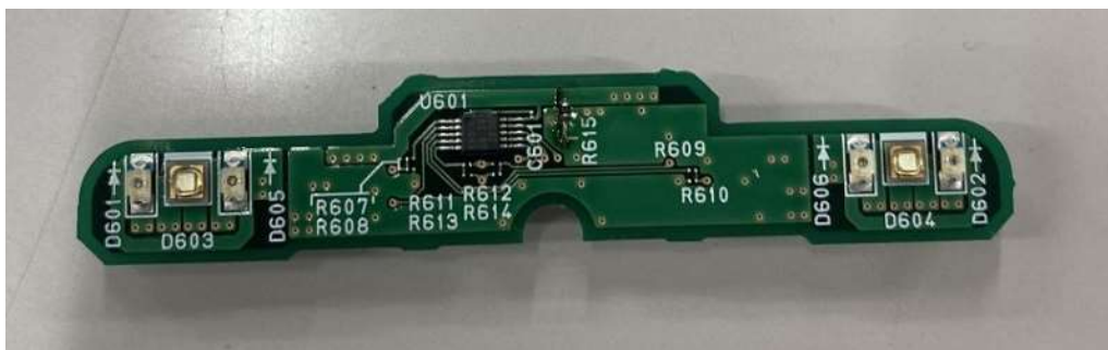
LED board_L front
