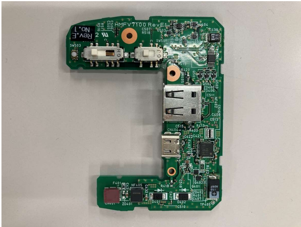
Sub board front
