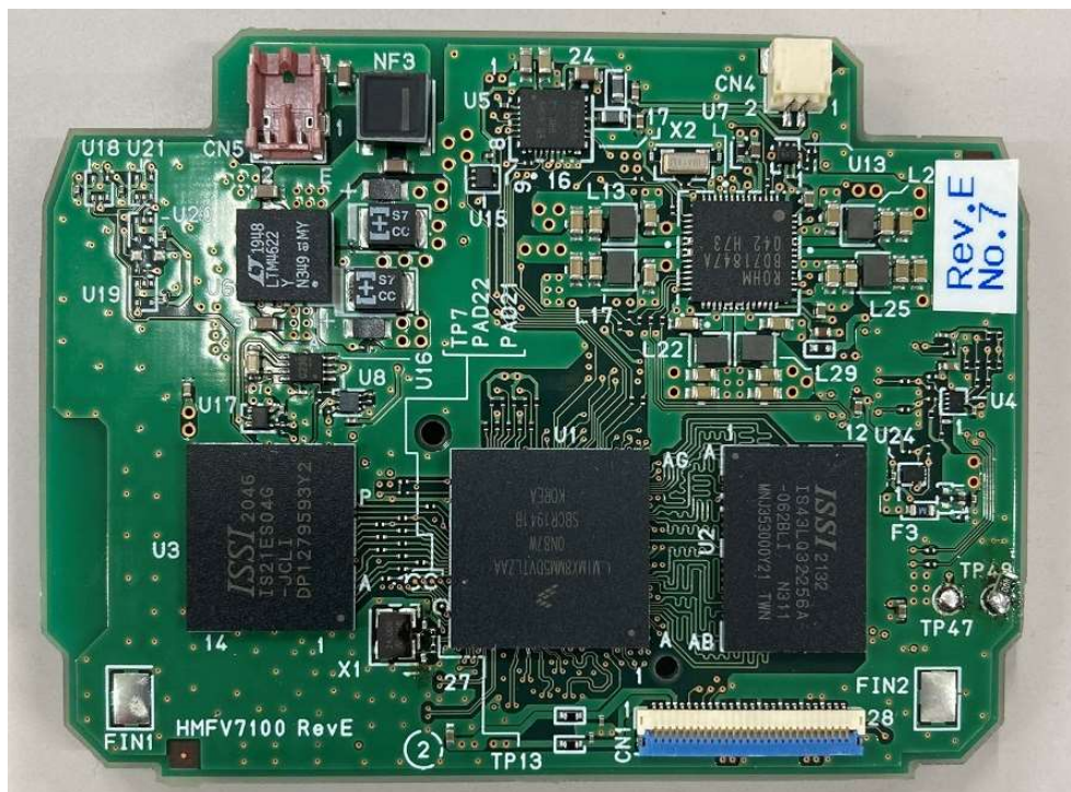
Main board front
