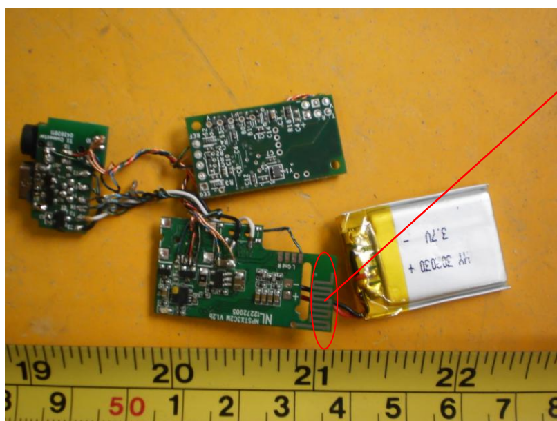
Main PCB photograph of EUT
