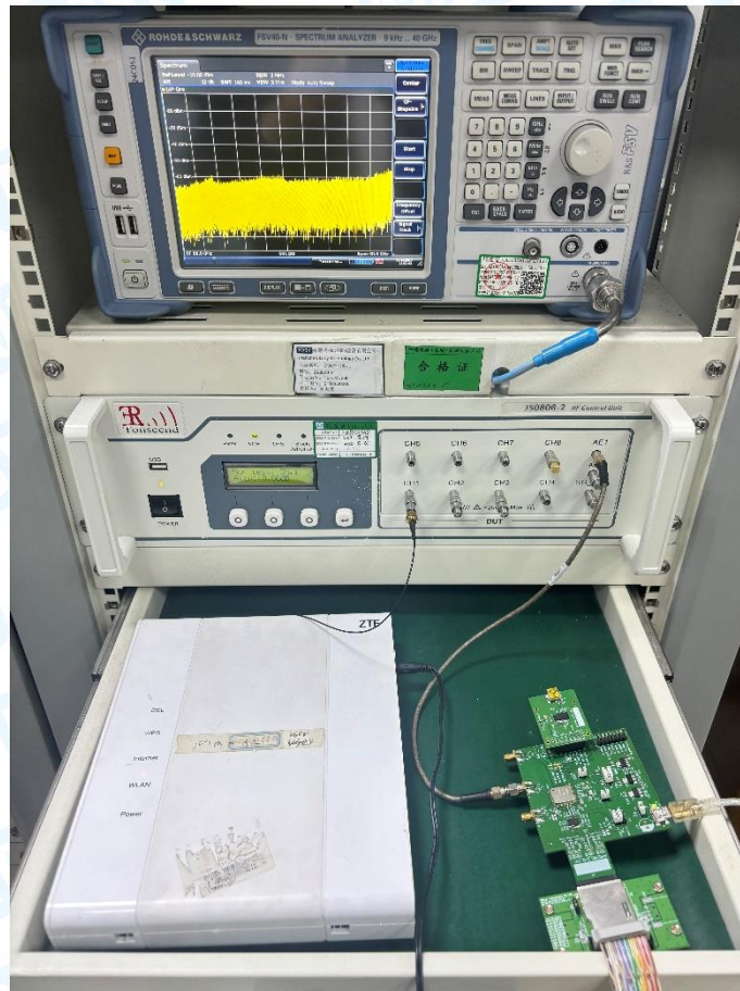
Photo of Setup for DFS Test
