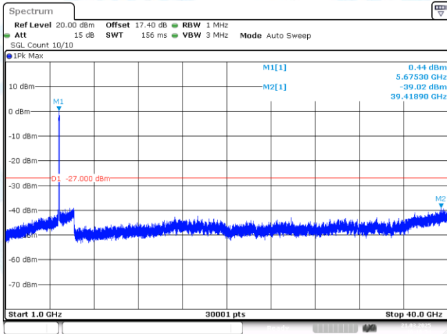
11AC80MIMO-Ant1-5690-1000~40000-PASS
