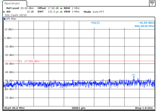
11AX20MIMO-Ant2-5260-30~1000-PASS
