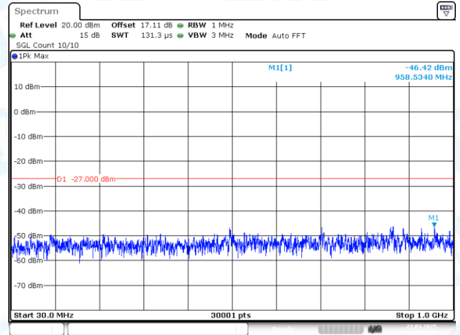
11AC40MIMO-Ant2-5510-30~1000-PASS
