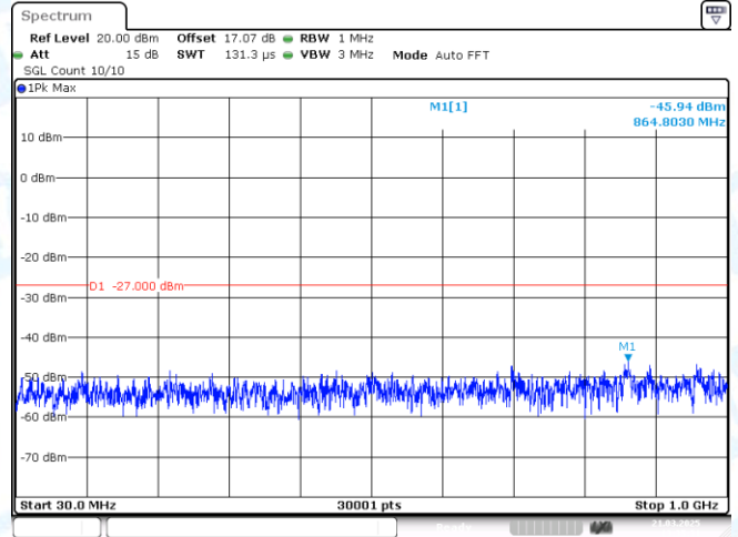
11AC40MIMO-Ant2-5230-30~1000-PASS
