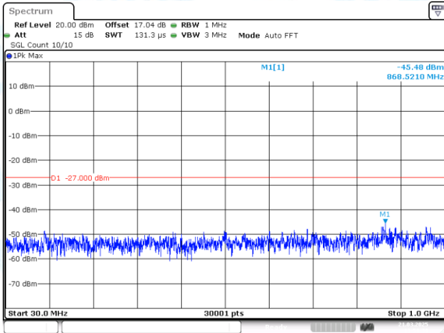
11AC40MIMO-Ant1-5510-30~1000-PASS
