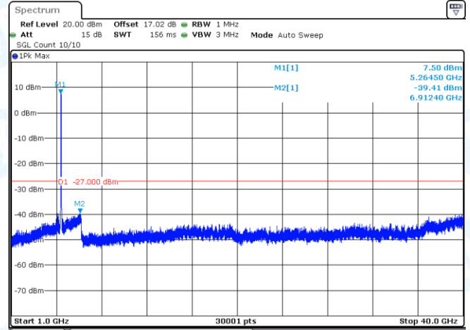
11AC40MIMO-Ant2-5270-1000~40000-PASS
