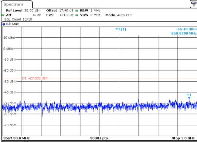
11AC40MIMO-Ant1-5710-30~1000-PASS
