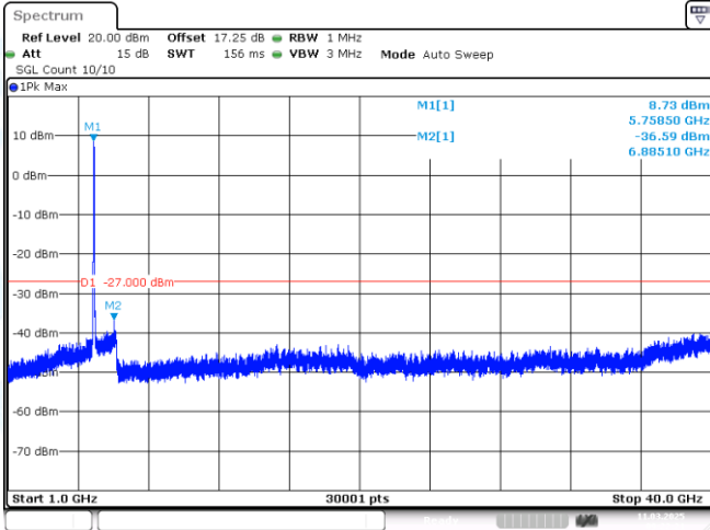
11AC40MIMO-Ant1-5755-1000~40000-PASS
