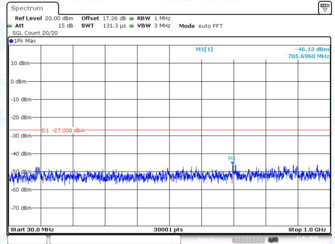
11AC20MIMO-Ant2-5785-30~1000-PASS
