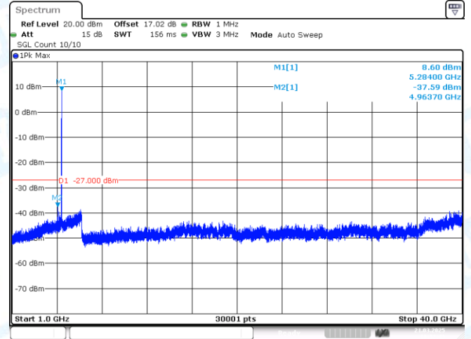
11AX20MIMO-Ant2-5280-1000~40000-PASS
