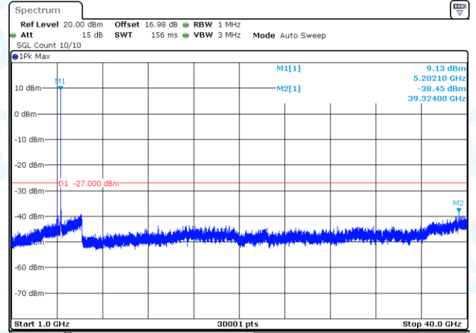
11AX20MIMO-Ant2-5200-1000~40000-PASS
