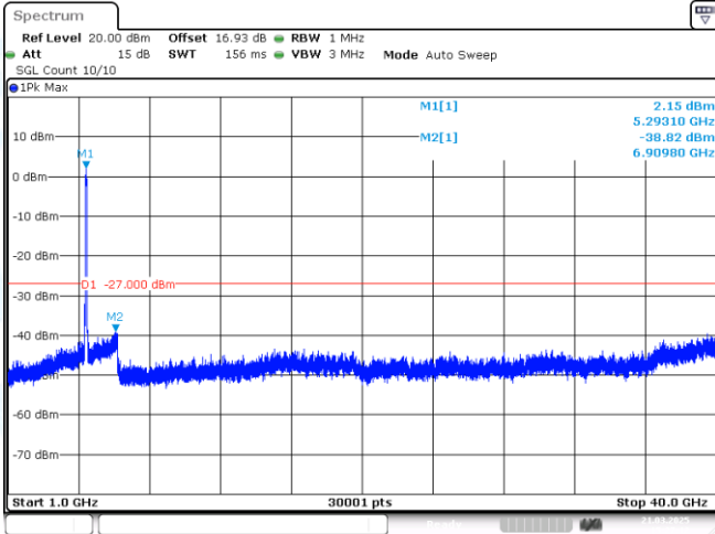
11AC80MIMO-Ant1-5290-1000~40000-PASS
