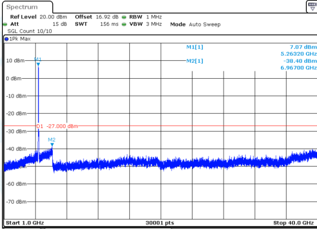
11AC40MIMO-Ant1-5270-1000~40000-PASS
