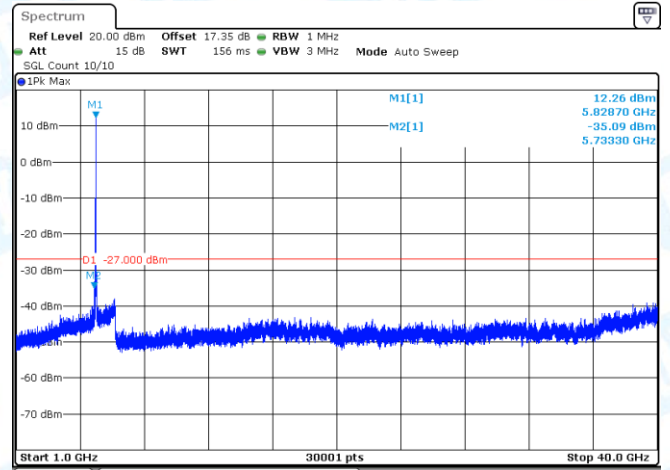
11AC20MIMO-Ant2-5825-1000~40000-PASS
