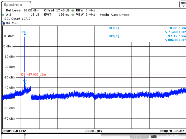
11AC20MIMO-Ant1-5720-1000~40000-PASS
