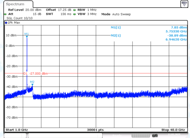
11AC40MIMO-Ant2-5755-1000~40000-PASS
