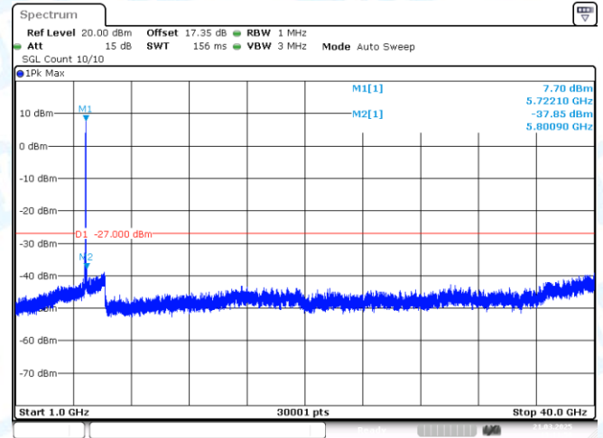
11AC20MIMO-Ant2-5720-1000~40000-PASS
