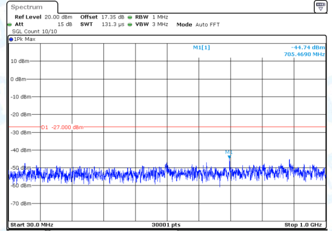
11AC40MIMO-Ant2-5710-30~1000-PASS
