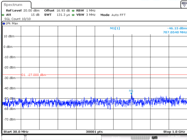
11AC20MIMO-Ant1-5320-30~1000-PASS
