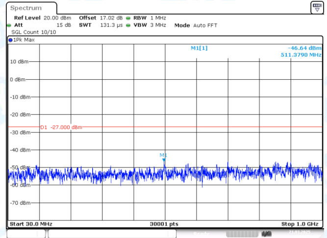
11AC20MIMO-Ant2-5320-30~1000-PASS
