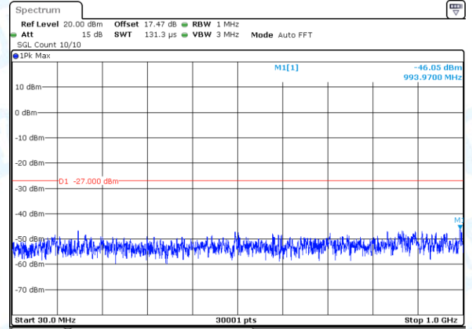
11N40MIMO-Ant2-5670-30~1000-PASS
