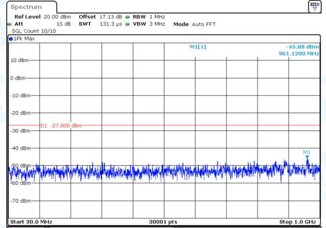
11N20MIMO-Ant2-5580-30~1000-PASS
