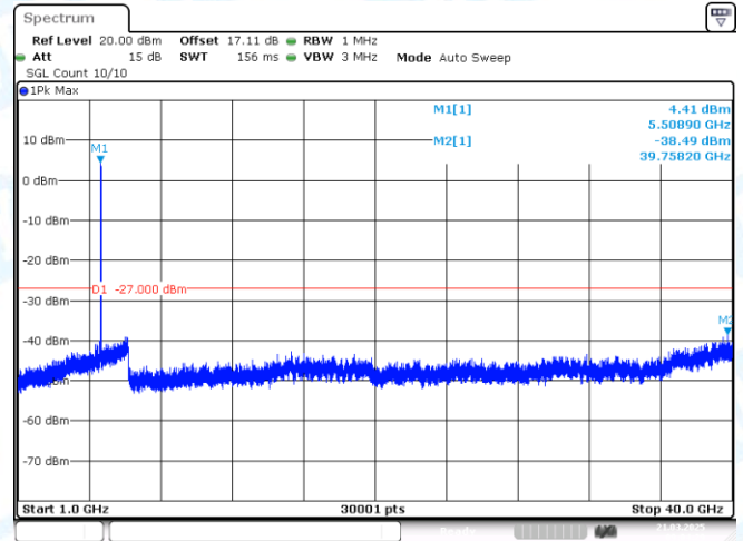
11N40MIMO-Ant2-5510-1000~40000-PASS
