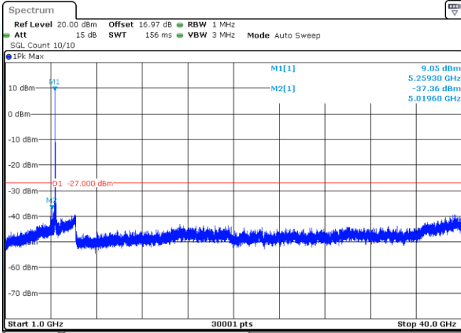
11AC20MIMO-Ant1-5260-1000~40000-PASS
