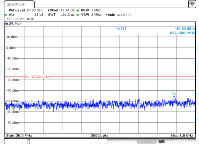
11AC20MIMO-Ant2-5700-30~1000-PASS
