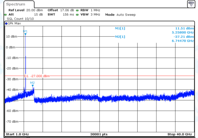
11AC20MIMO-Ant2-5260-1000~40000-PASS
