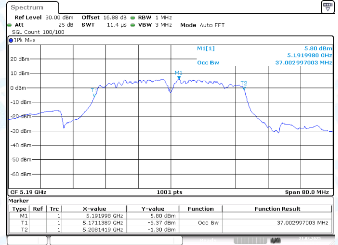
11AC40MIMO-Ant1-5190
