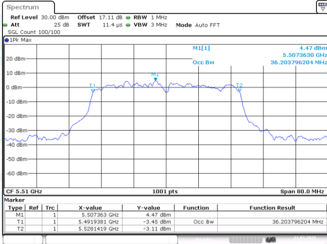
11N40MIMO-Ant2-5510
