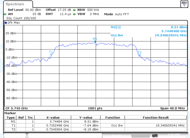
11AC20MIMO-Ant1-5745
