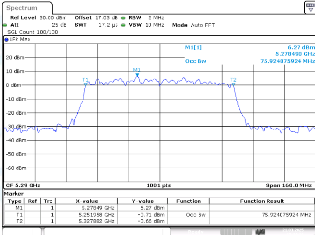
11AC80MIMO-Ant2-5290
