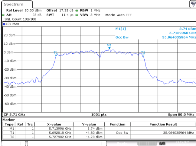
11N40MIMO-Ant2-5710
