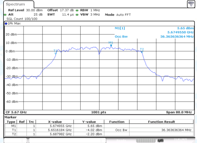
11AC40MIMO-Ant1-5670
