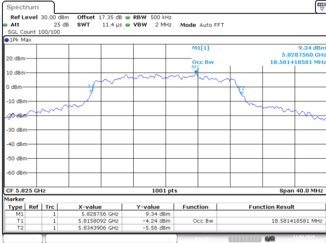
11AC20MIMO-Ant2-5825
