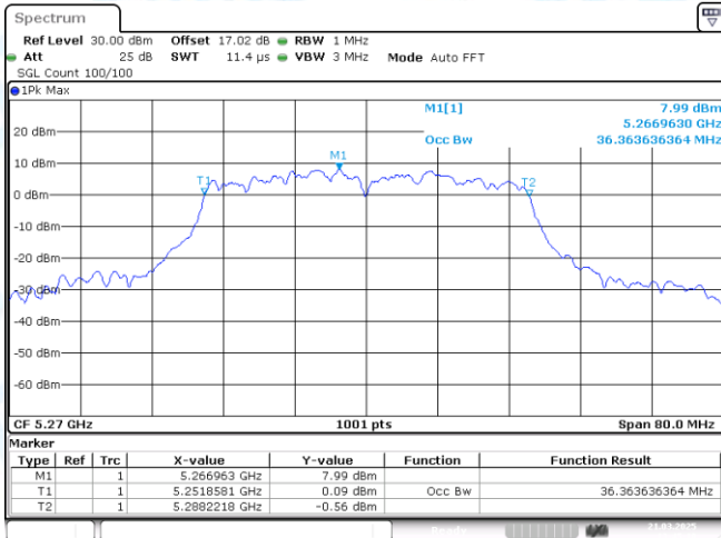
11AC40MIMO-Ant2-5270
