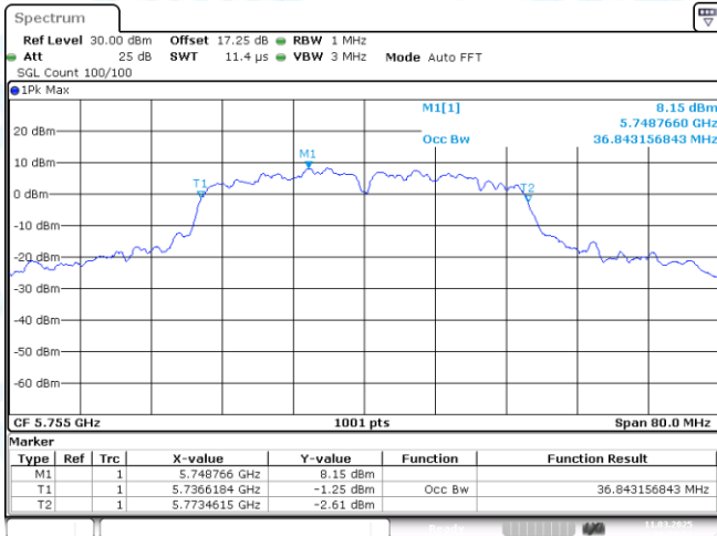
11AC40MIMO-Ant2-5755
