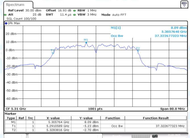
11AC40MIMO-Ant1-5310
