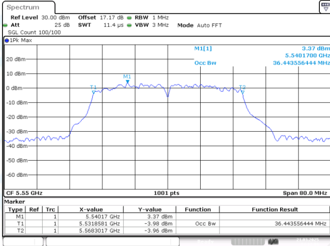
11AC40MIMO-Ant2-5550
