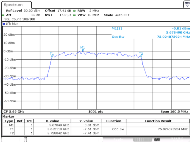
11AC80MIMO-Ant2-5690
