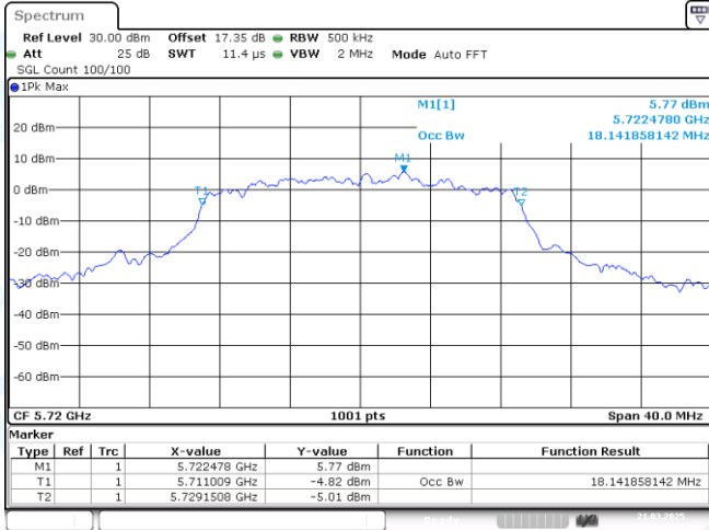
11AC20MIMO-Ant2-5720
