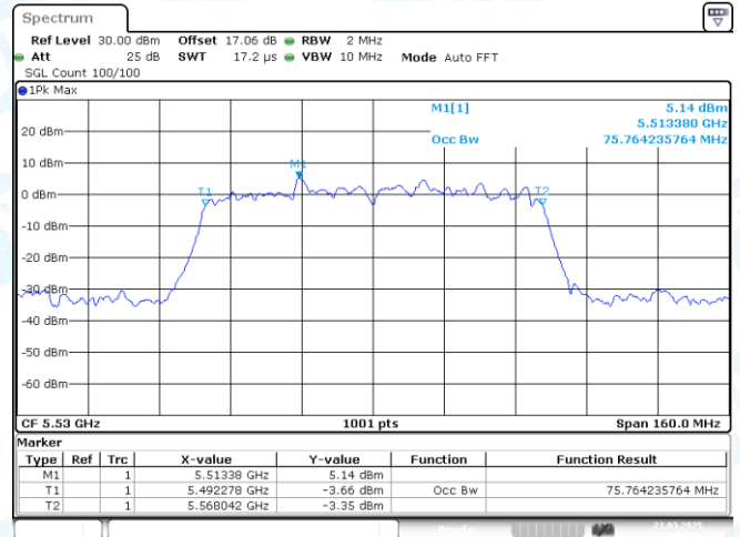
11AC80MIMO-Ant1-5530
