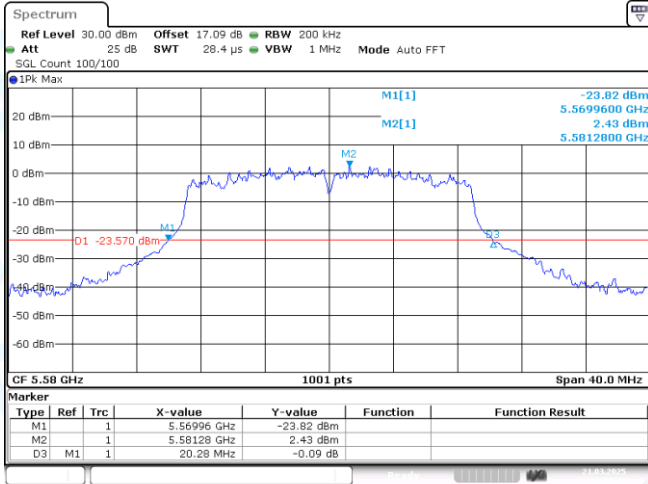
11AC20MIMO-Ant1-5580
