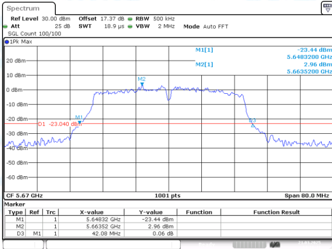
11AC40MIMO-Ant1-5670
