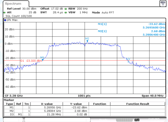
11AC20MIMO-Ant2-5280
