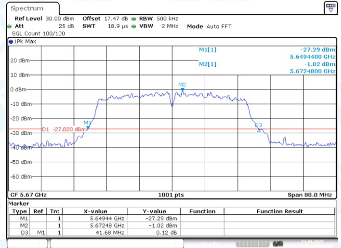
11AC40MIMO-Ant2-5670
