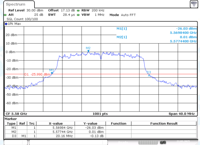
11AC20MIMO-Ant2-5580
