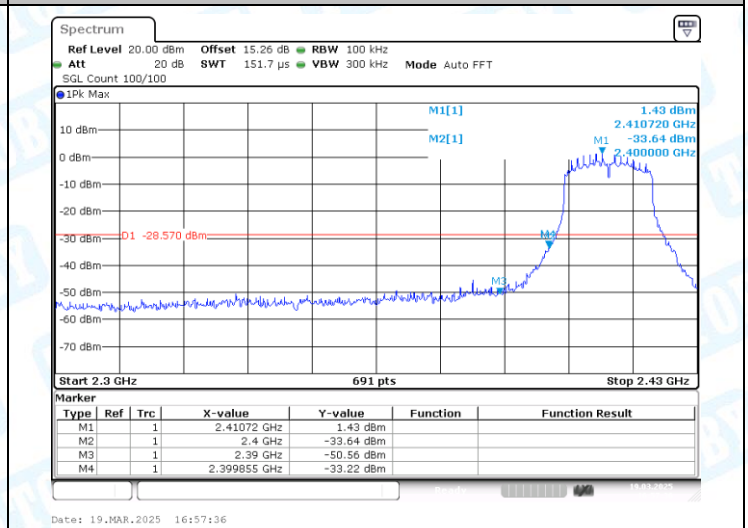
11N20MIMO-Ant2-2412-PASS
