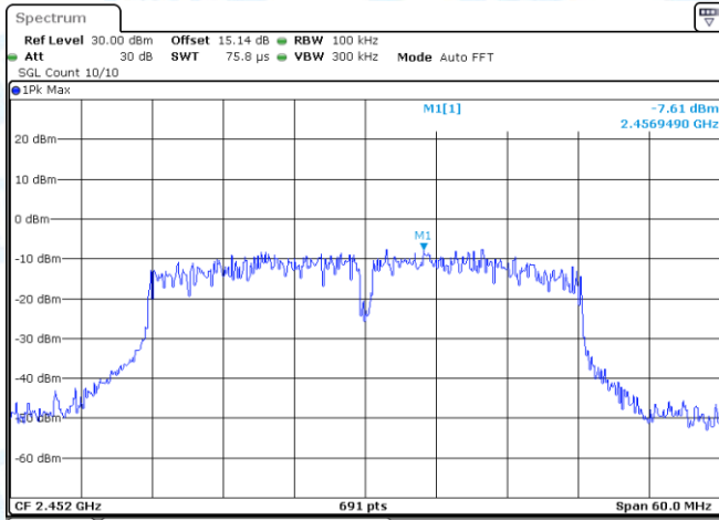
11N40MIMO-Ant1-2452-0~Reference-PASS
