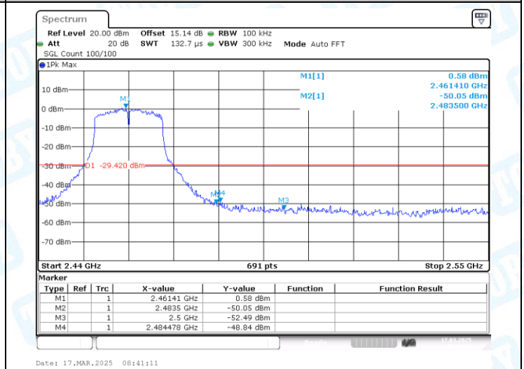
11G-Ant1-2462-PASS
