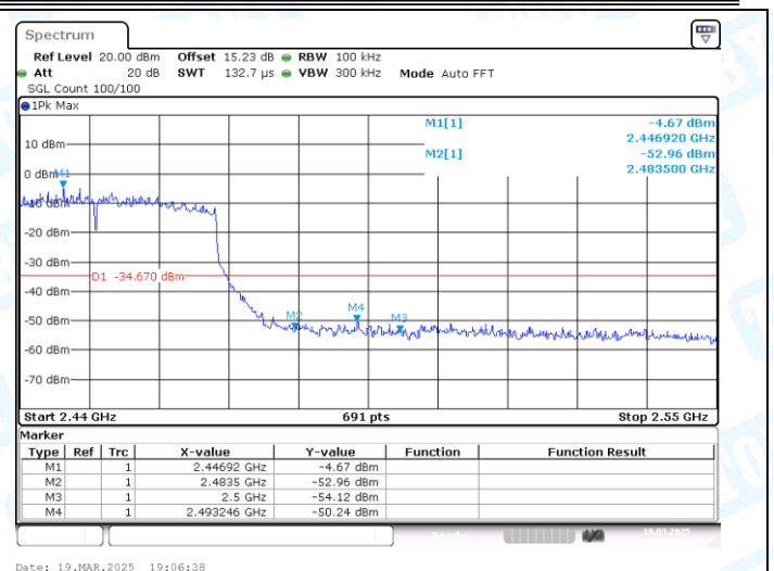
11AX40MIMO-Ant2-2452-PASS
