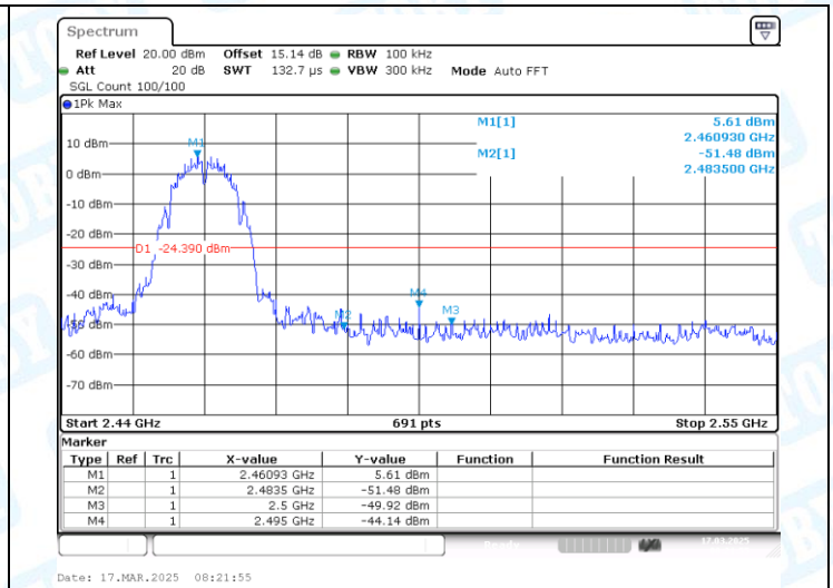
11B-Ant1-2462-PASS
