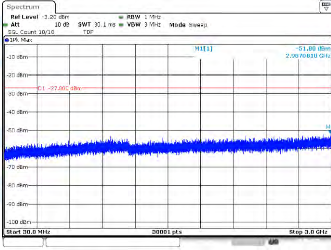
11AX40SISO-Ant1-6445-30~3000-PASS
