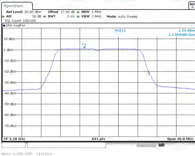
11AC20SISO-Ant1-5280-PASS
