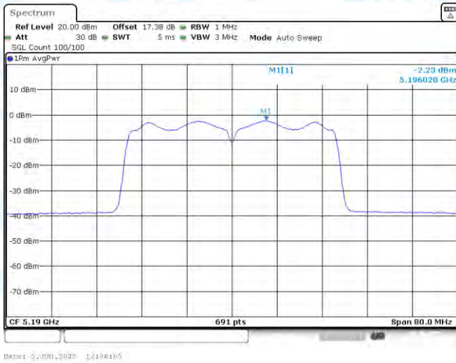
11N40SISO-Ant1-5190-PASS
