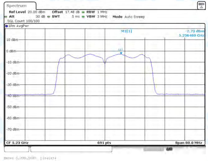
11N40SISO-Ant1-5230-PASS
