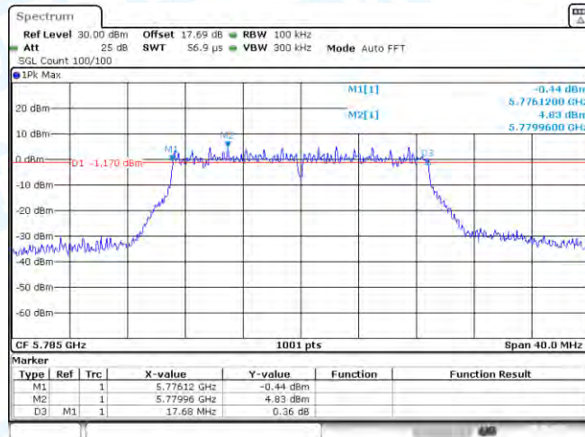
11AC20SISO-Ant1-5785-PASS
