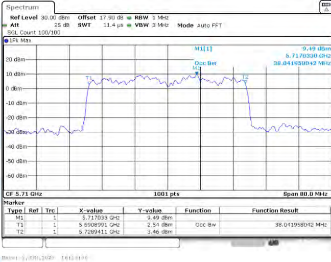
11AX40SISO-Ant1-5710
