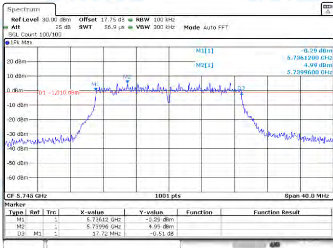
11AC20SISO-Ant1-5745-PASS
