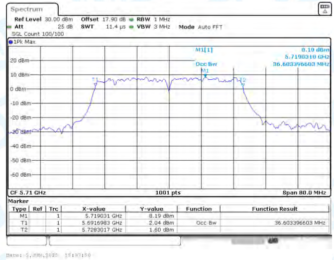
11AC40SISO-Ant1-5710
