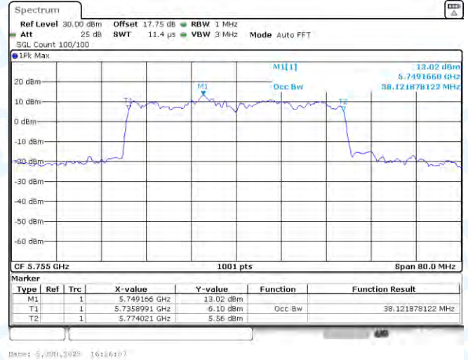
11AX40SISO-Ant1-5755
