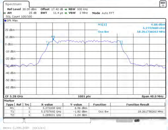
11AC20SISO-Ant1-5280
