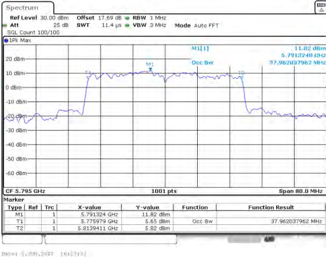
11AX40SISO-Ant1-5795
