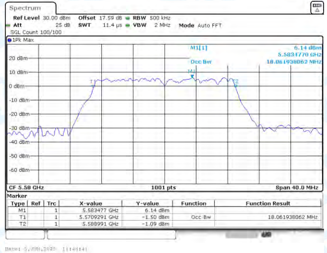
11N20SISO-Ant1-5580
