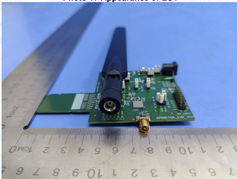
Photo 17 Appearance of EUT
