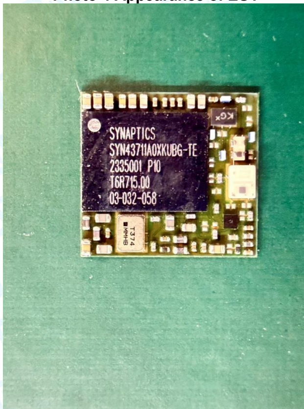
Photo 4 Appearance of EUT
