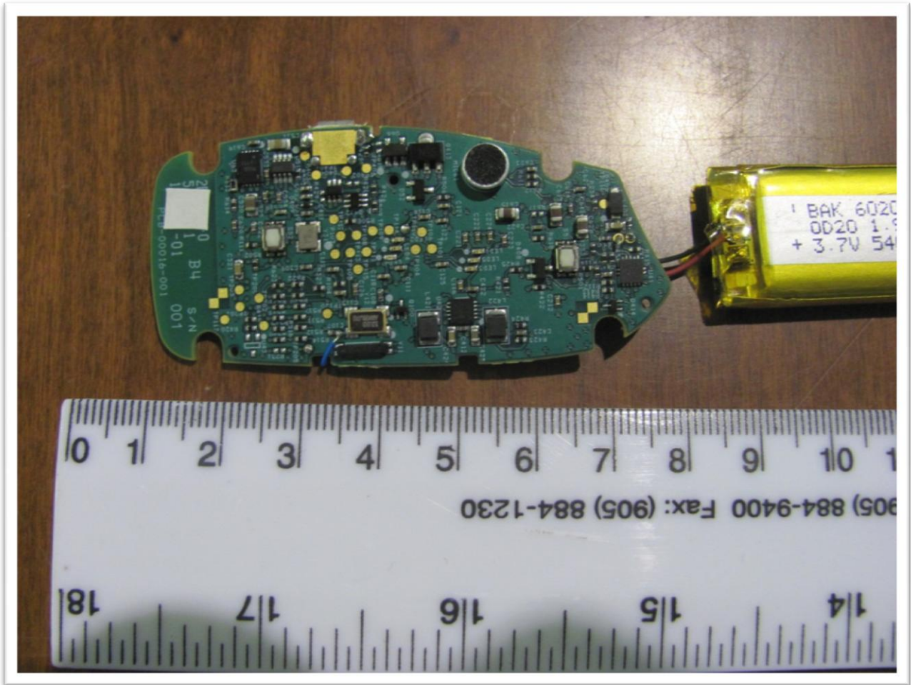
Figure 4 – EUT PCB Bottom
