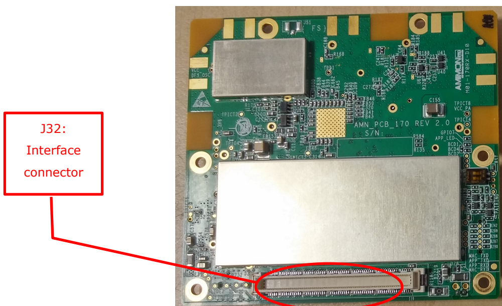
Figure 2 – Rx 670TS0029 bottom side
