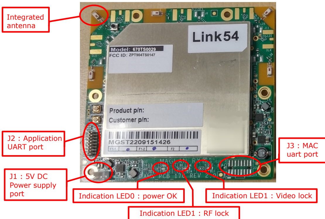
Figure 1 – Rx 670TS0029 top-side
