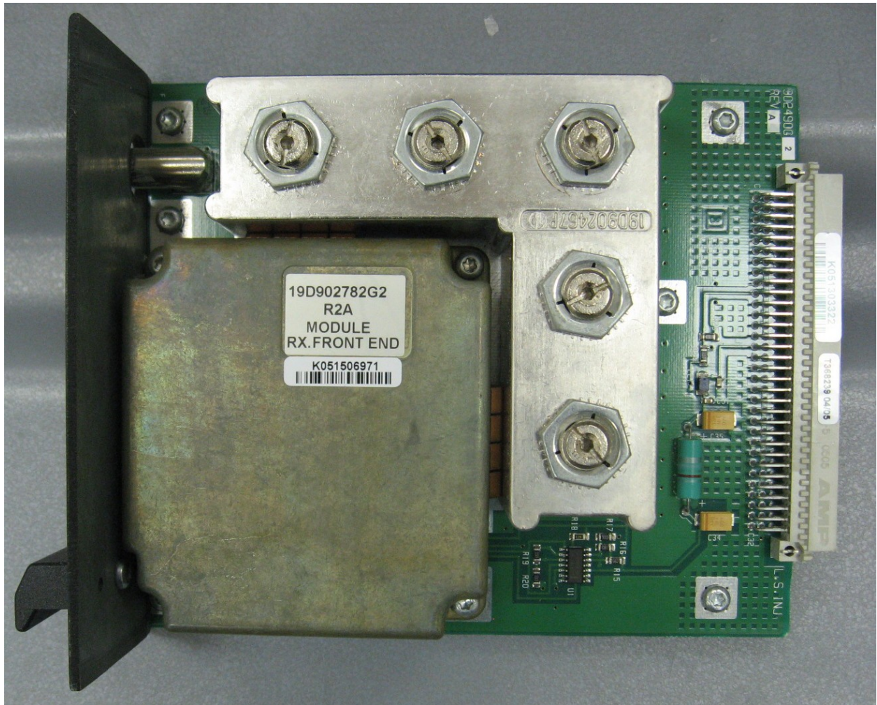
Figure 8 RX Front End
