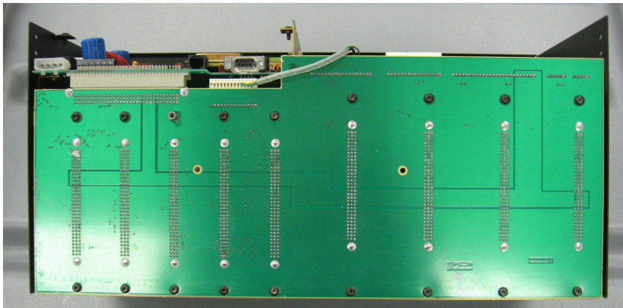
Figure 3 Mastr3 Rear View
