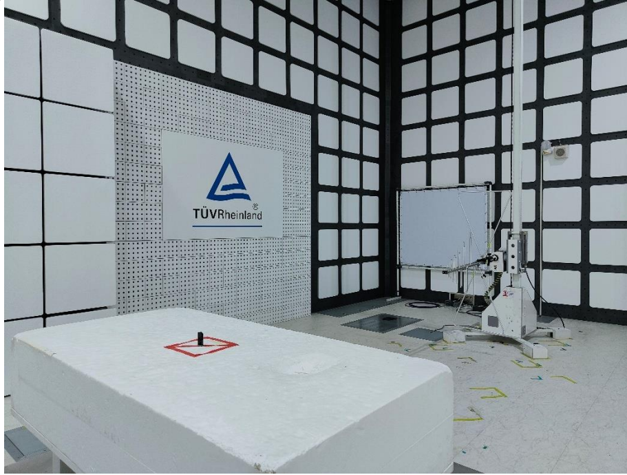
Photograph 12: Test Setup for Spurious Emissions (Back View 3, FSK Mode)
