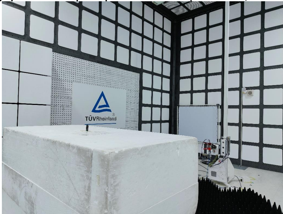
Photograph 6: Test Setup for Spurious Emissions (Back View 3, ASK Mode)
