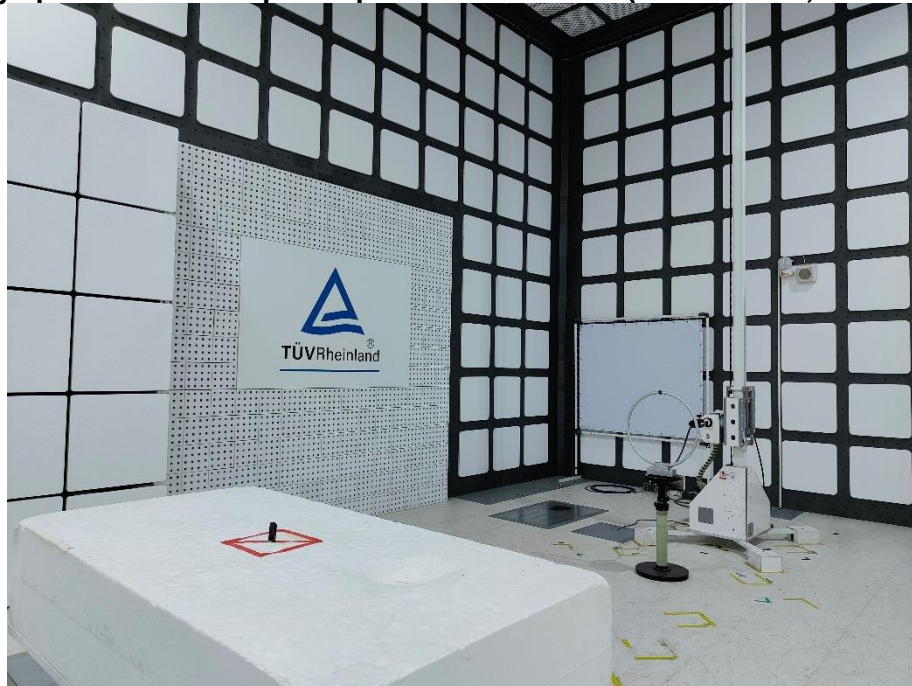
Photograph 10: Test Setup for Spurious Emissions (Back View 1, FSK Mode)
