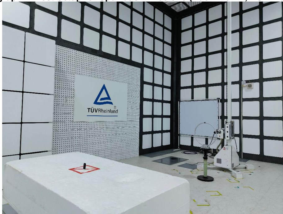
Photograph 4: Test Setup for Spurious Emissions (Back View 1, ASK Mode)
