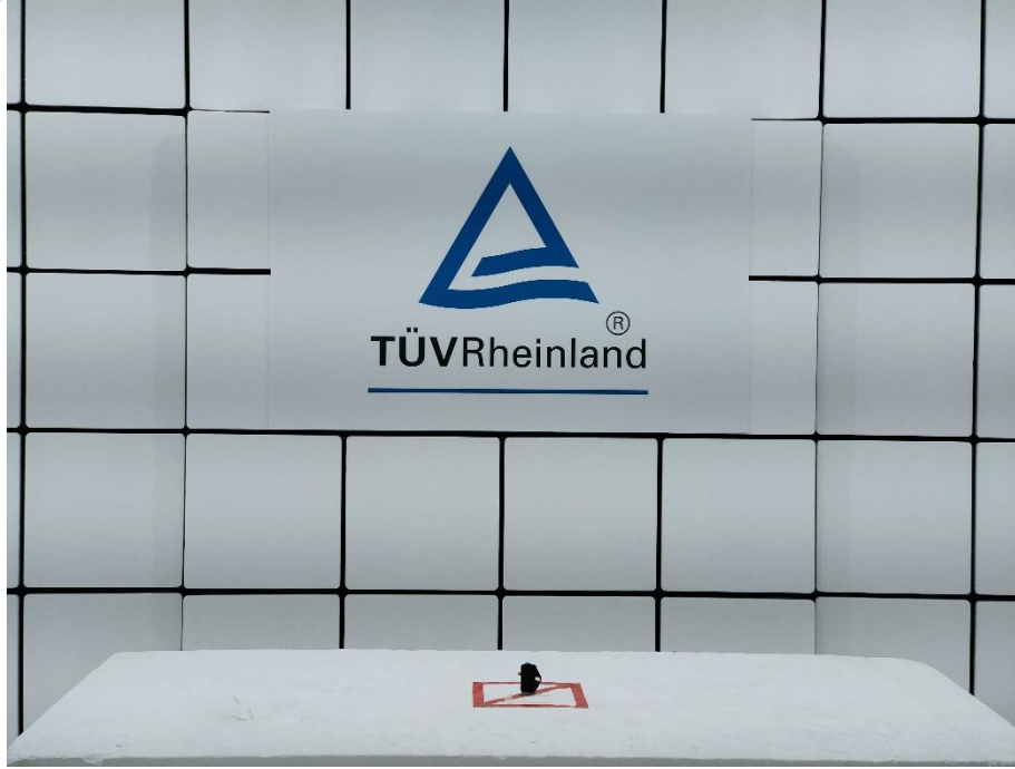
Photograph 2: Test Setup for Spurious Emissions (Front View 2, ASK Mode)
