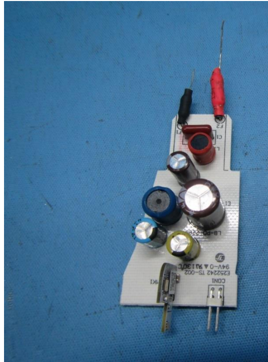
Driver PCB view
