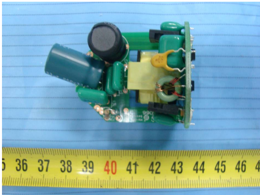
EUT – All Main Board Side View
