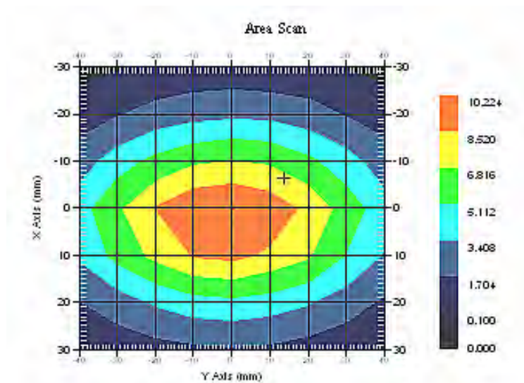
835 MHz System Validation with Body Tissue
