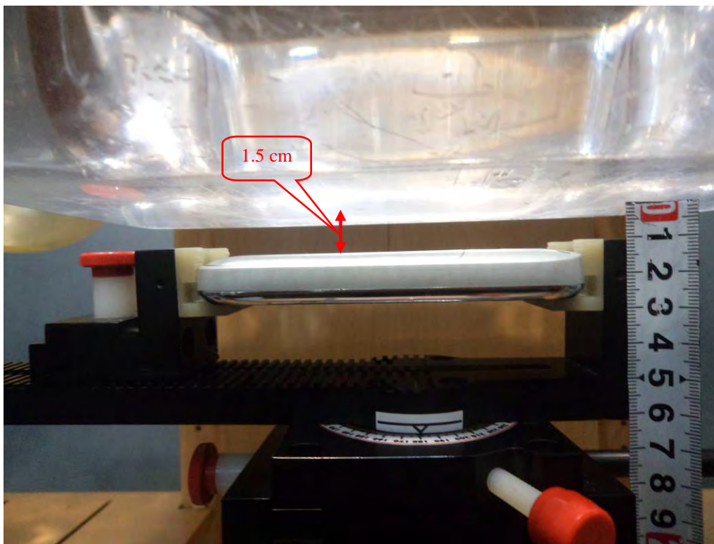
Wi-Fi Body Position D Setup Photo
