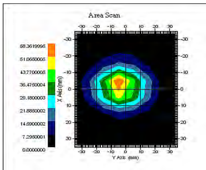
2450 MHz System Validation with Head Tissue
