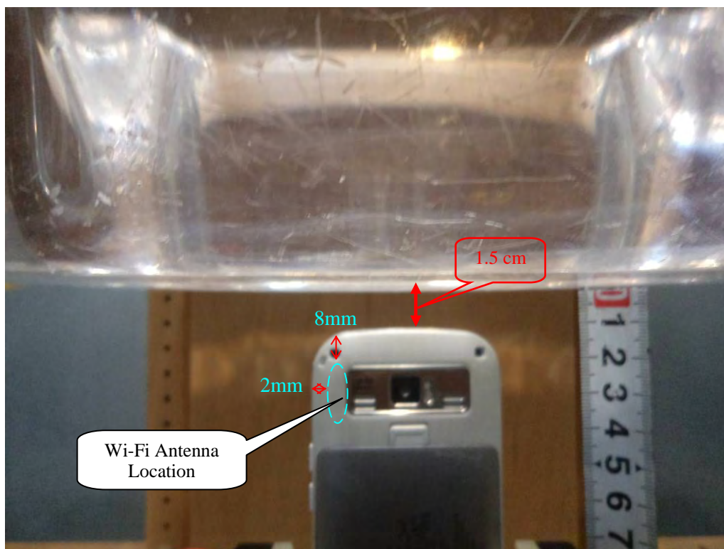
Wi-Fi Body Position B Setup Photo
