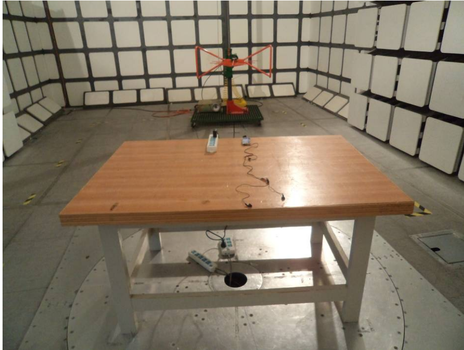
Radiated Emissions –Front View (charging & media playing mode)
